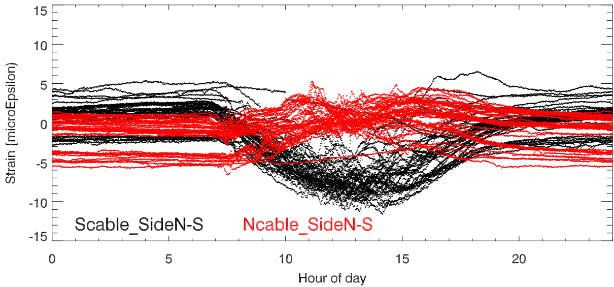
StrainDif (Side1 - Side2) vs Hour of day. Platform Tower 8
