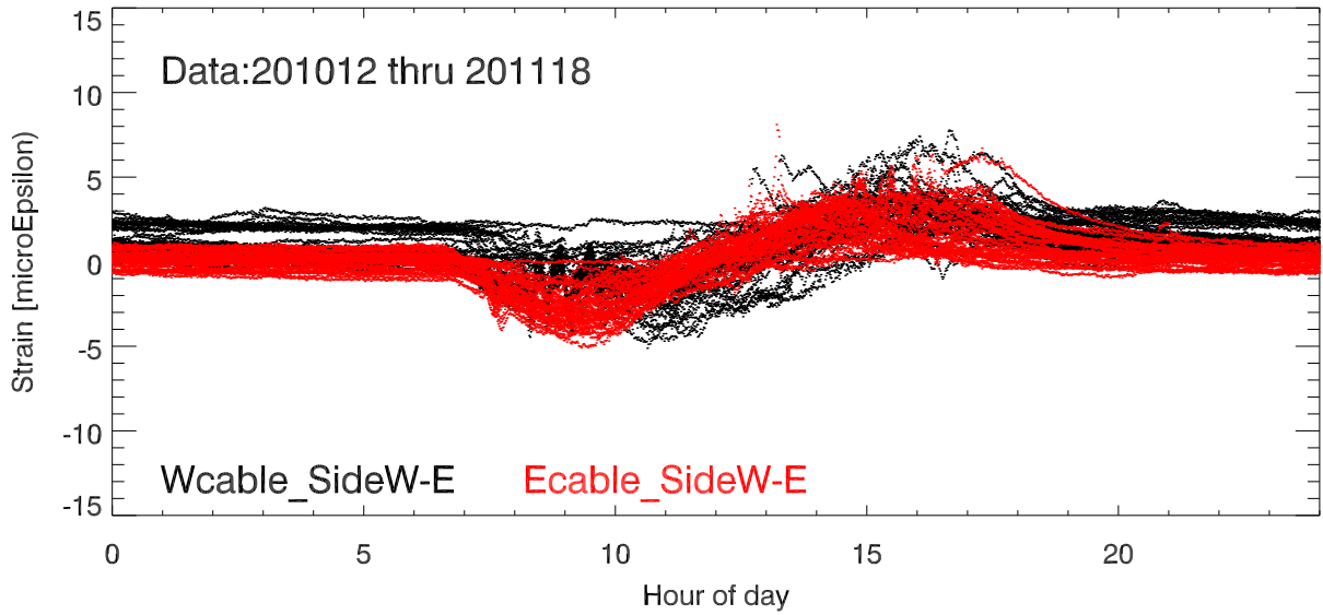
StrainDif (Side1 - Side2) vs Hour of day. Platform Tower 12
