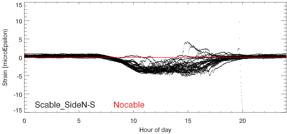
StrainDif (Side1 - Side2) vs Hour of day. Platform Tower 4
