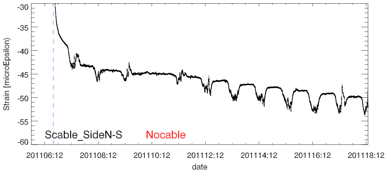
StrainDif (Side1 - Side2) vs date. Platform Tower 4
