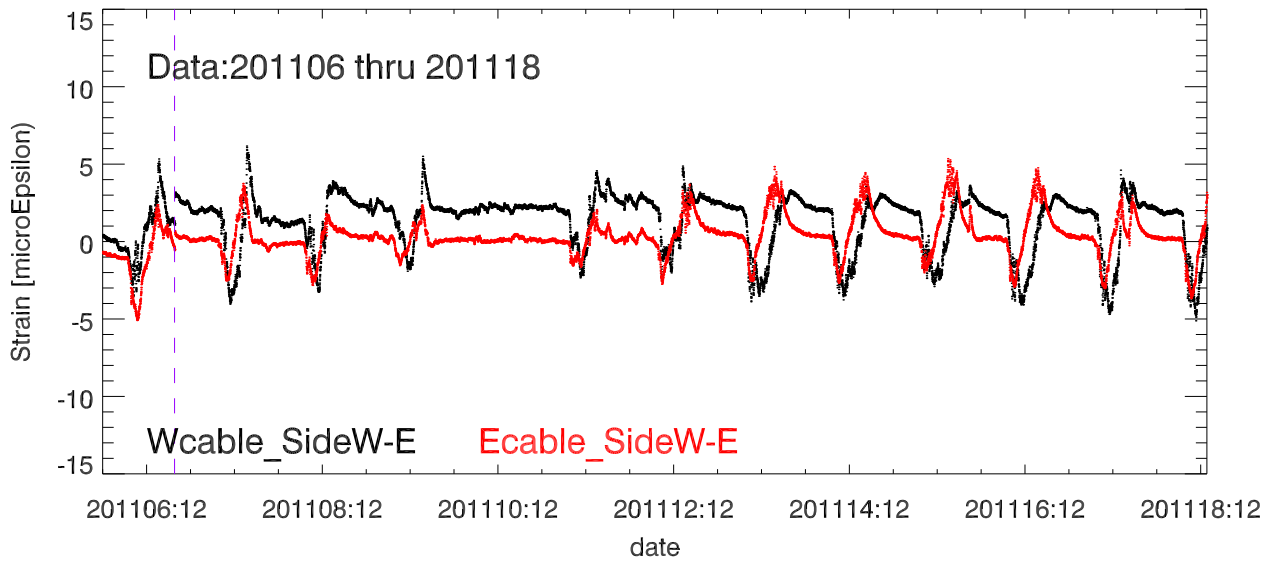
StrainDif (Side1 - Side2) vs date. Platform Tower 12
