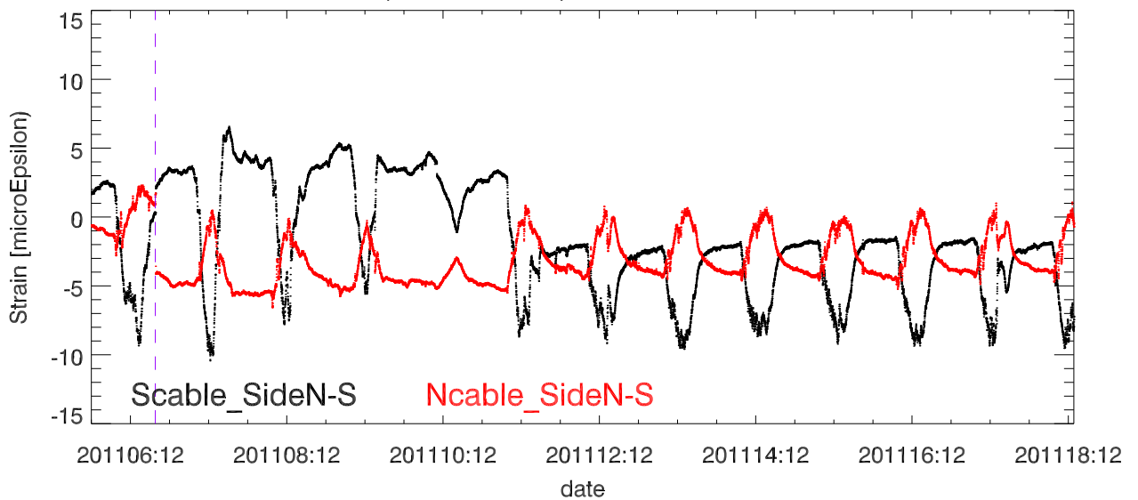
StrainDif (Side1 - Side2) vs date. Platform Tower 8
