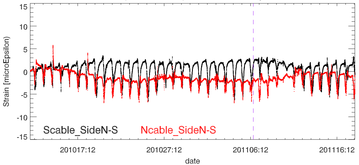
StrainDif (Side1 - Side2) vs date. BackStay Tower 4
