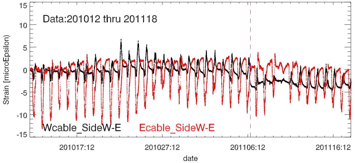
StrainDif (Side1 - Side2) vs date. BackStay Tower 12
