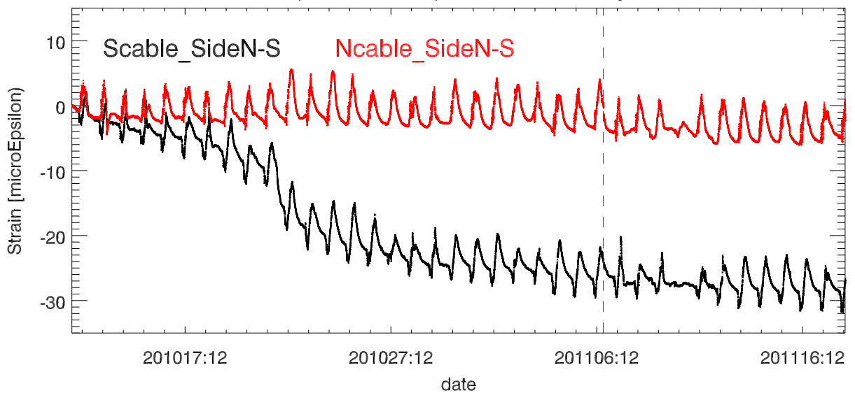
StrainDif (Side1 - Side2) vs date. BackStay Tower 8
