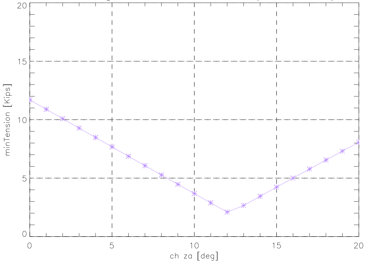
Ch tracking: min Td tension vs Ch za. (Dome at stow)
