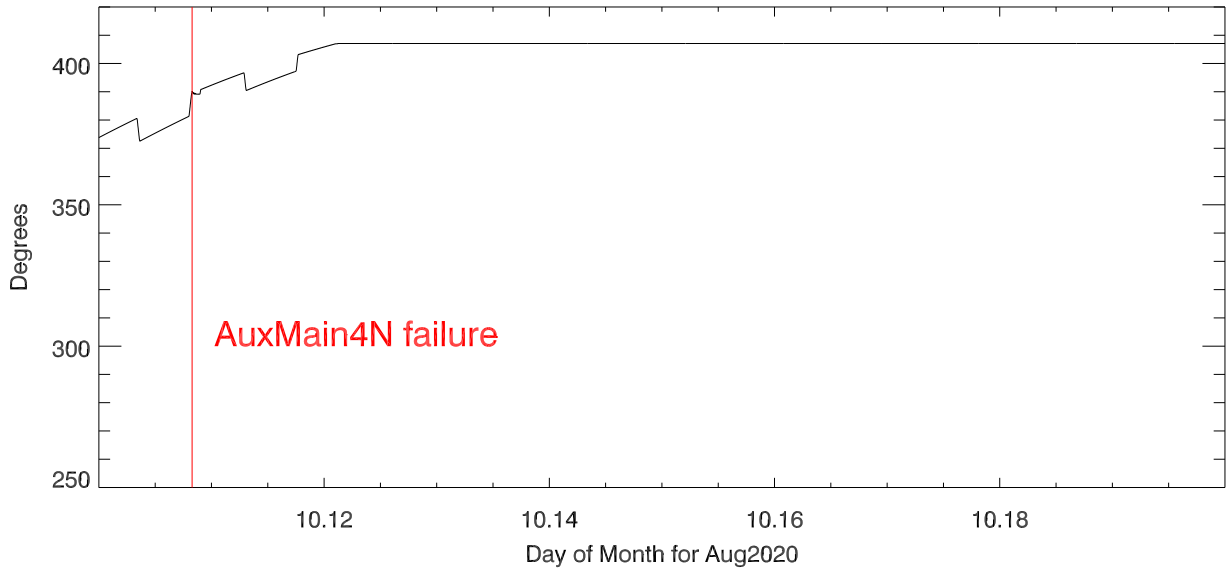
Azimuth position during auxmain4N failure
