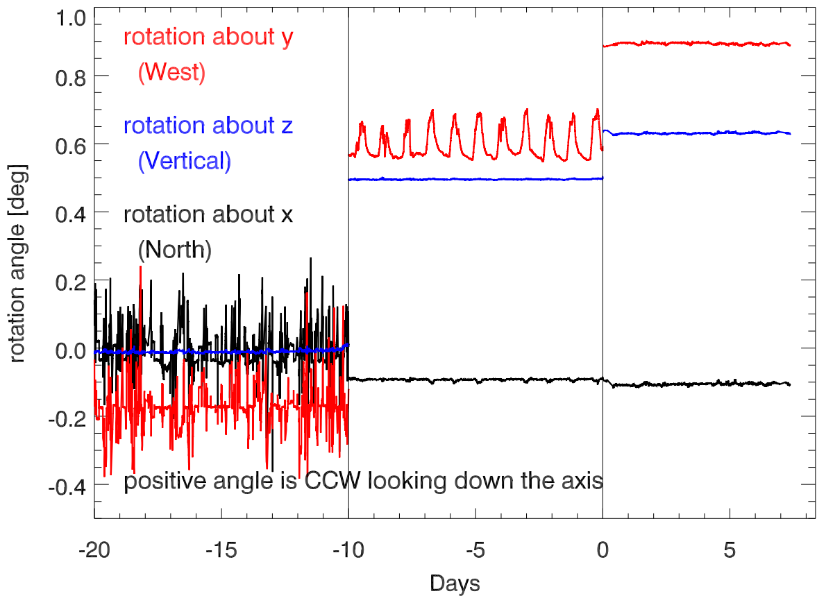
Platform rotation angles about x(north),y(west),z(vertical)
