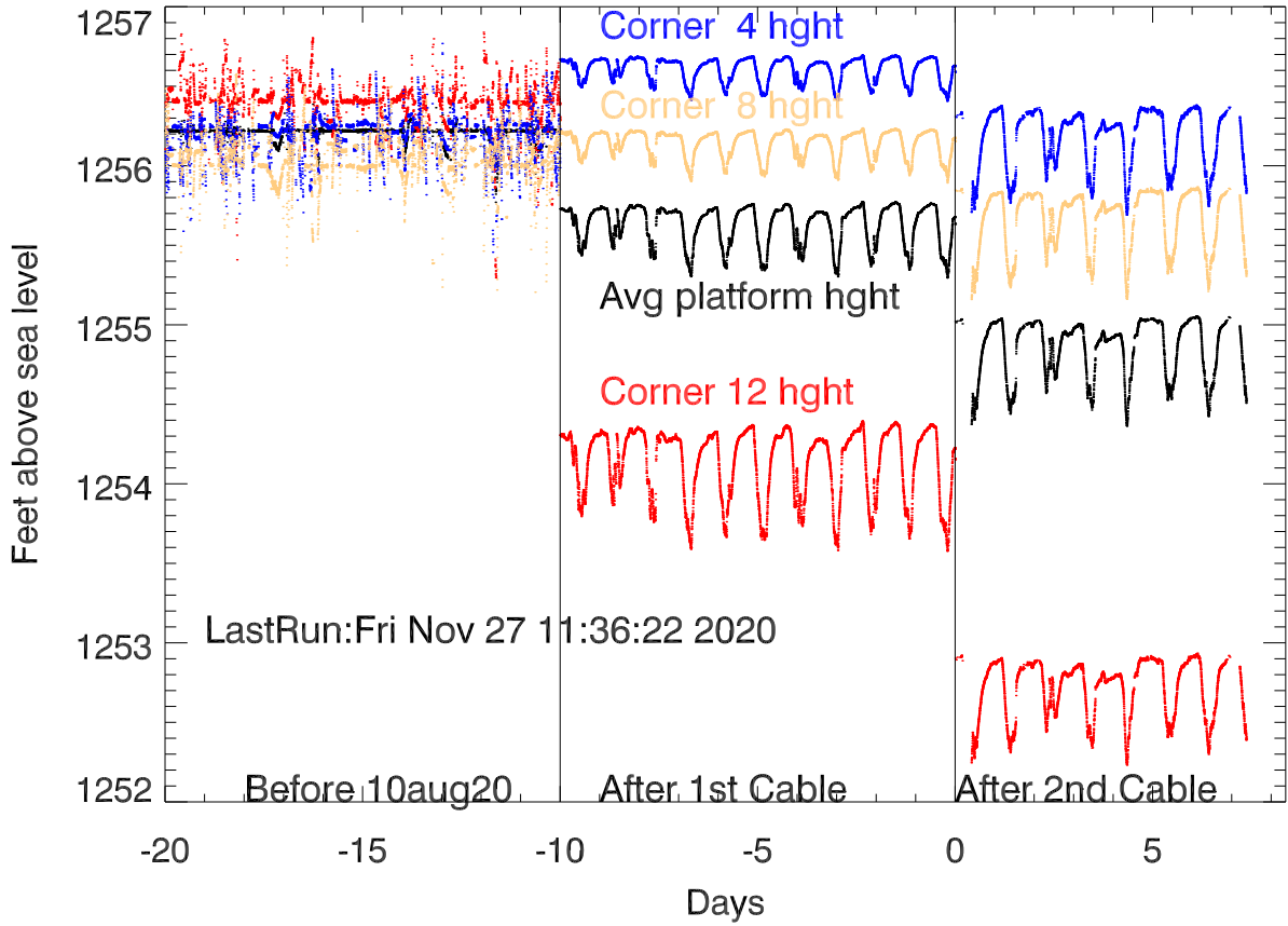
Platform Avg & corner Heights during cable failures
