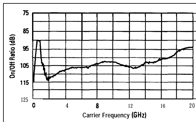
Figure 1-27. Typical Pulse Modulation On/Off Ratio at +8 dBm
