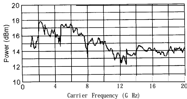
Figure 1-6. Typical Maximum Available Output Power from 1 to 20 GHz, at 25°C with Output Step Attenuator (Option 1E1) Installed
