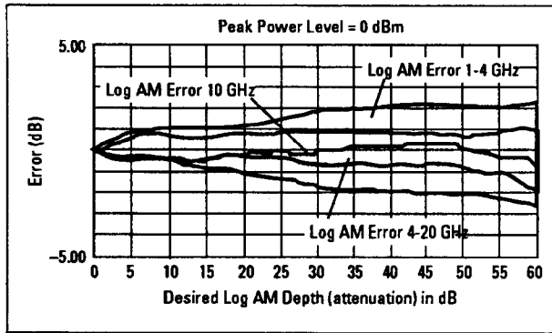
Figure 1-29. Typical Log AM Error (deviation from desired depth) at 25 °C for Carrier Frequencies between 1.0 and 20 GHz
