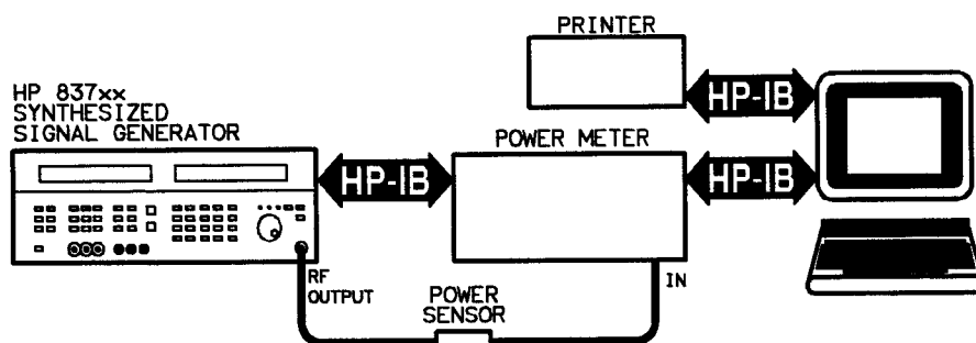
Figure 7-10. 0.01—1 GHz Frequency Calibration 1 Equipment Setup
