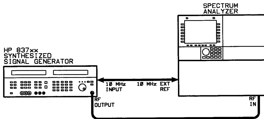
Figure 3-13. Pulse On/Off Ratio Test Setup
