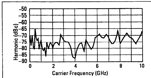
Figure 1-4. Typical 2nd Harmonic Levels Measured at Output Power of + 6 dBm
