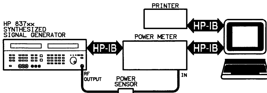
Figure 7-4. 1—20 GHz Frequency Calibration 2 Equipment Setup
