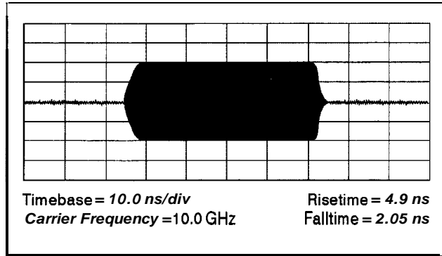
Figure 1-19. Typical Pulse Modulation Envelope Illustrates the Fast Rise and Fall Times, Excellent Flatness and Pulse Fidelity
