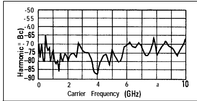
Figure 1-25. Typical 2nd Harmonic Levels Measured at Output Power of + 6 dBm
