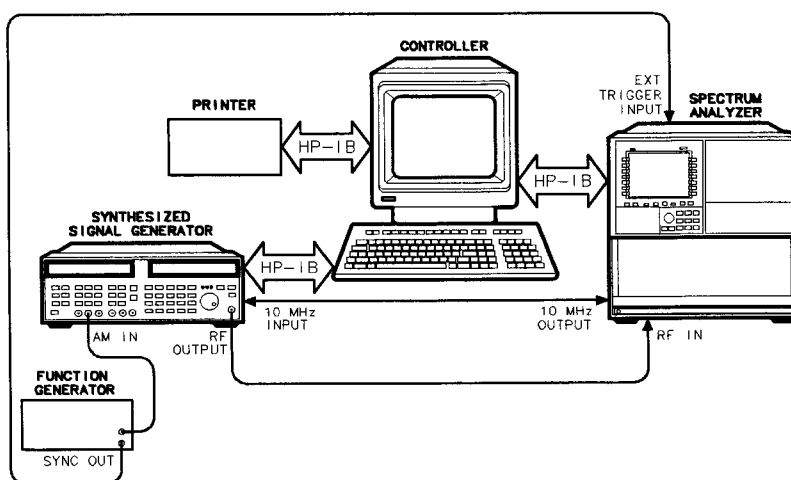
Figure 7-6. 1—20 GHz AM Linearity Calibration Equipment Setup
