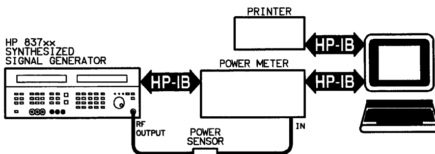
Figure 7-9. 0.01—1 GHz Vernier Calibration Equipment Setup
