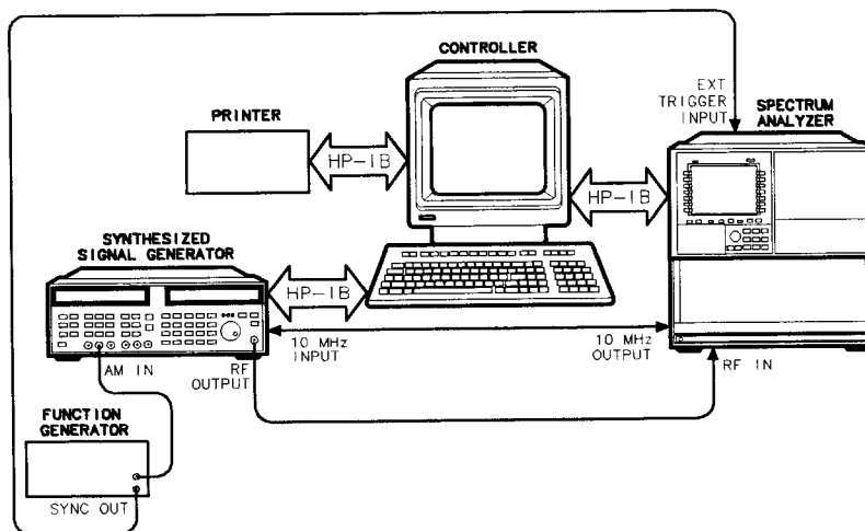
Figure 7-13. 0.01—1 GHz AM Calibration Equipment Setup
