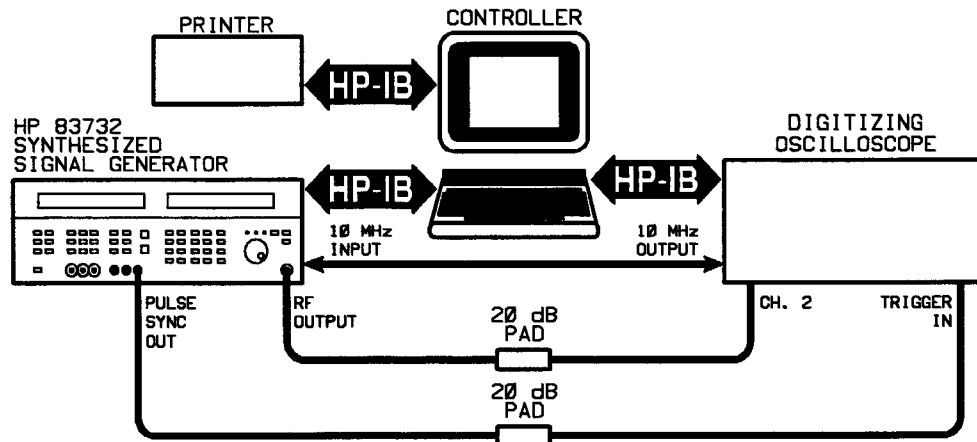
Figure 7-15. 0.01—1 GHz Pulse Calibration Equipment Setup
