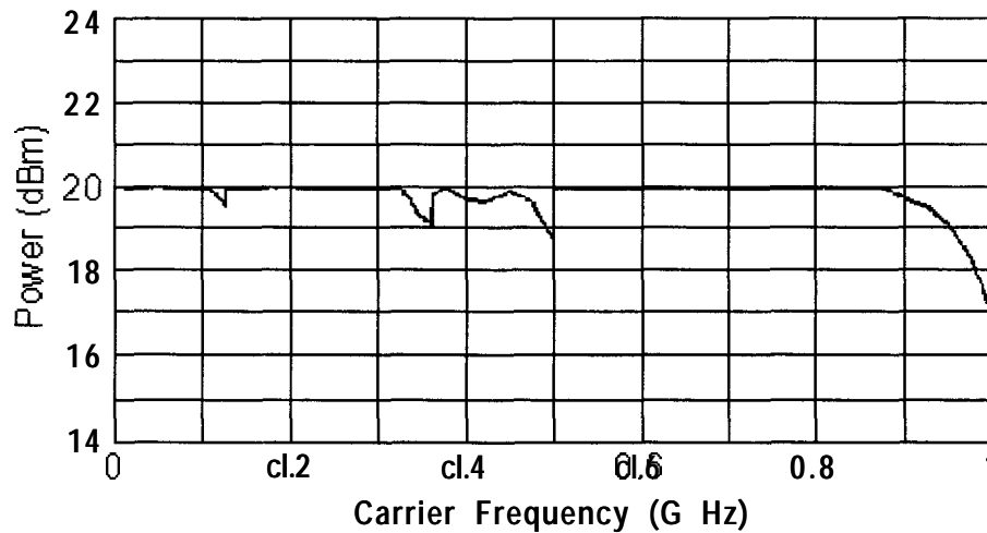
Figure 1-22. Typical Maximum Available Output Power from 0.01 to 1 GHz at 25 °C
