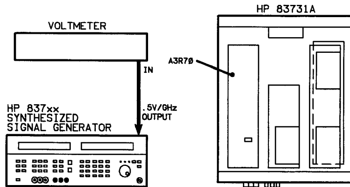
Figure 6-4. 0.5 V/GHz Output Equipment Setup
