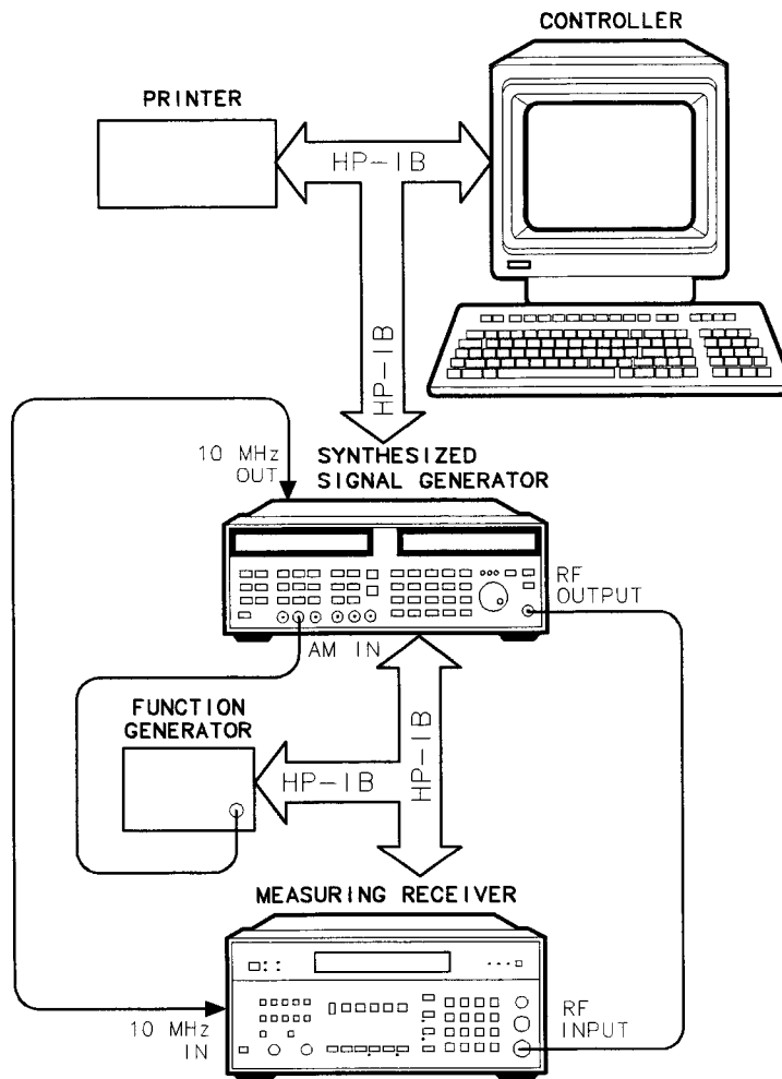
Figure 7-14. 0.01—1 GHz Linear AM Calibration Equipment Setup
