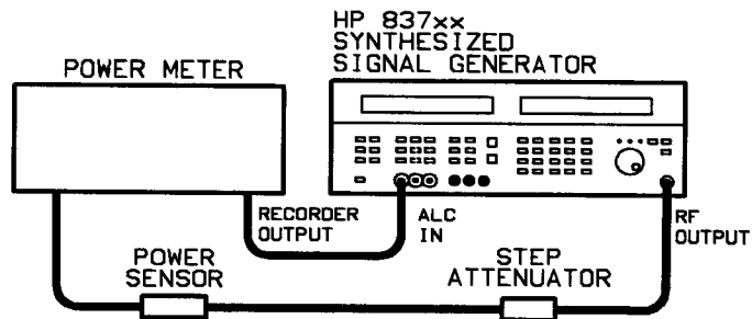
Figure 3-3. External Leveling Test Setup
