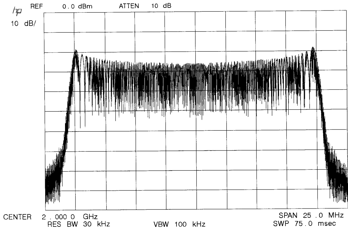
Figure 3-20. Example Signal Spectrum that Passes Test
