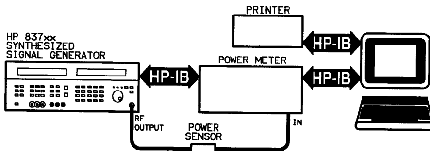
Figure 7-11. 0.01—1 GHz Frequency Calibration 2 Equipment Setup
