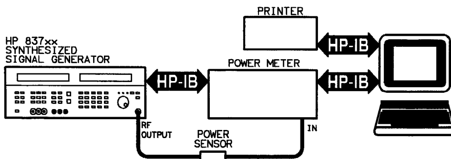
Figure 7-3. 1—20 GHz Frequency Calibration Equipment Setup
