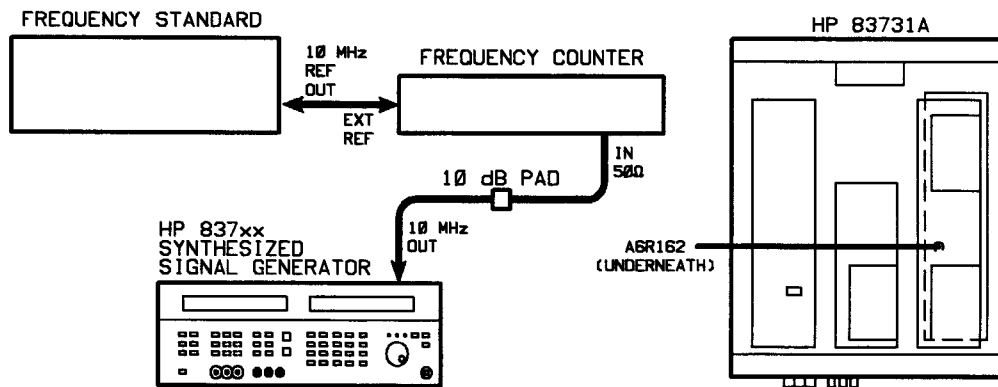
Figure 6-3. Low Stability Timebase Equipment Setup
