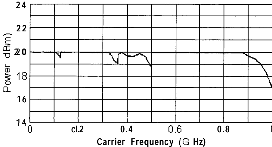
Figure 1-7. Typical Maximum Available Output Power from 0.01 to 1 GHz at 25°C
