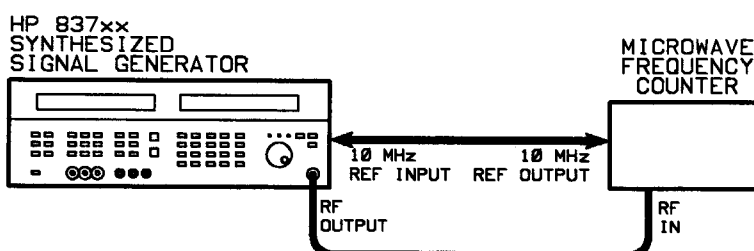
Figure 3-2. Frequency Range and Resolution Test Setup
