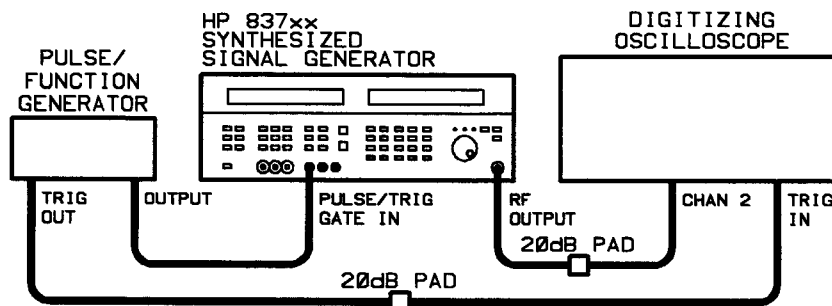
Figure 3-17. Pulse Width Test Setup
