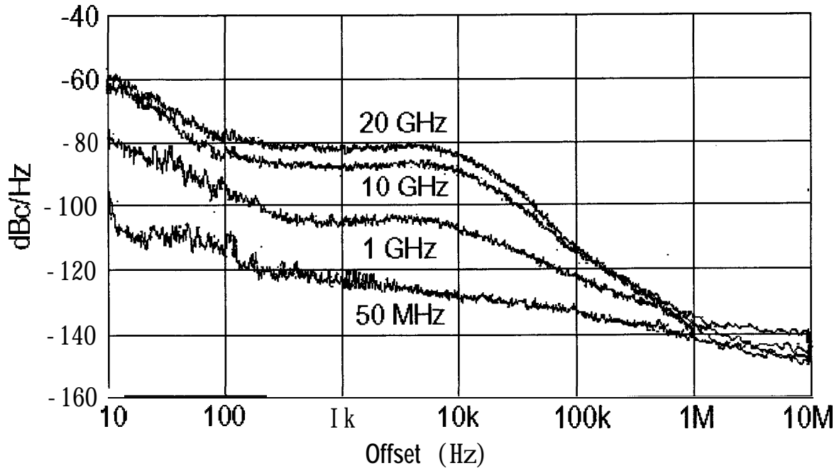
Figure 1-3. Typical single-sideband phase noise at 1 GHz, 10 GHz and 20 GHz, 25°C, CW mode. Offsets less than 100 Hz require the high stability timebase, Option 1E5.
