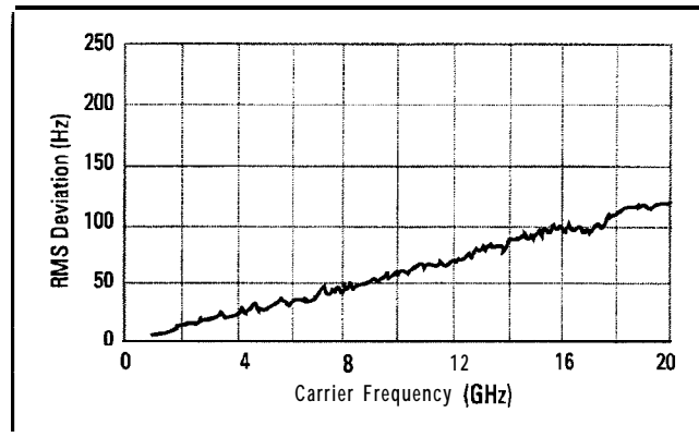
Figure 1-5. Typical Residual FM Measured in 50 Hz - 15 kHz Bandwidth, CW Mode, with High Stability Timebase (Option 1E5)
