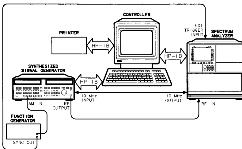
Figure 7-7. 1–20 GHz Log AM Gain Calibration Equipment Setup
