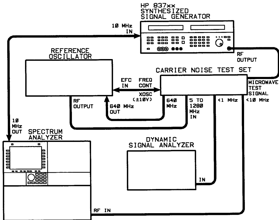
Figure 3-11. Non-Harmonic Spurious Level <30 kHz Test Setup
