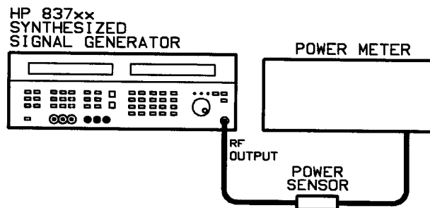
Figure 3-6. Low Level Accuracy Test Setup using Power Meter
