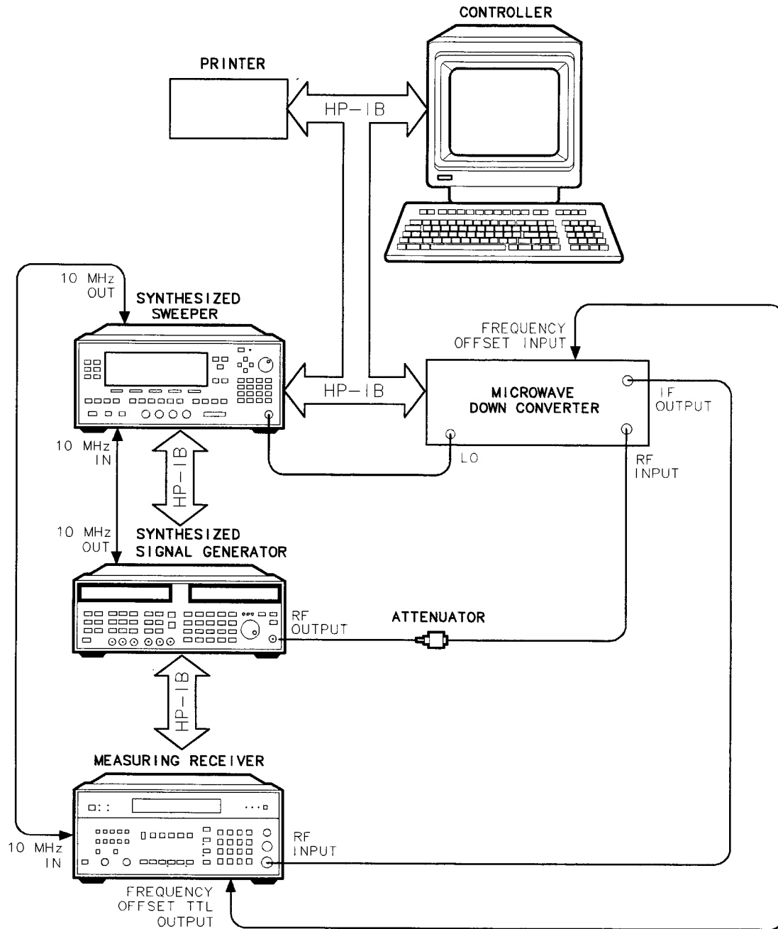
Figure 7-5. 1–20 GHz Attenuator Calibration Equipment Setup
