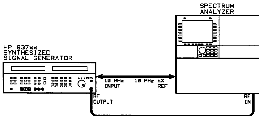
Figure 3-12. Non-Harmonic Spurious Level >30 kHz Test Setup
