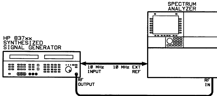
Figure 3-27. Internal FM Source Verification Test Setup
