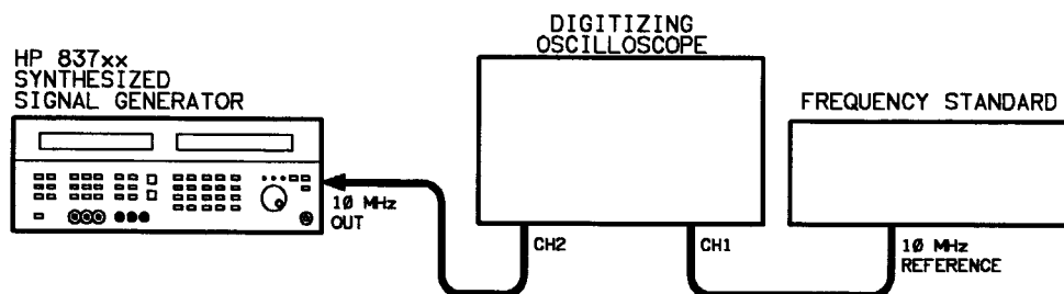
Figure 6-2. High Stability Timebase Adjustment Equipment Setup
