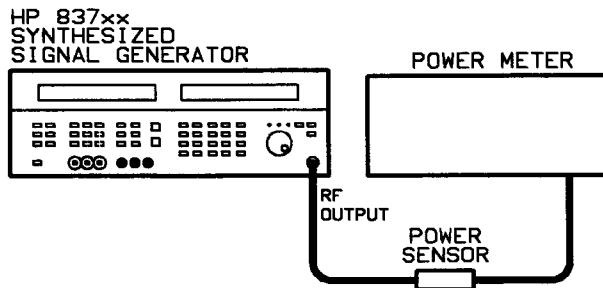
Figure 3-5. Vernier Level Accuracy and Flatness Test Setup
