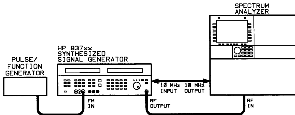
Figure 3-19. Maximum FM Deviation Test Setup
