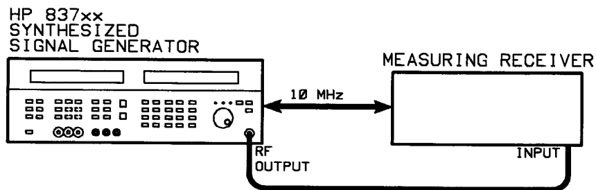
Figure 3-7. 10 MHz to 1 GHz Low Level Accuracy Test Setup using Measuring Receiver
