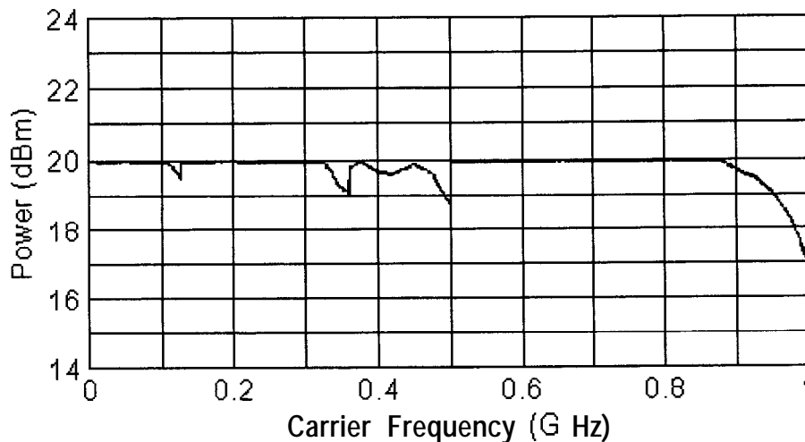
Figure 1-13. Typical Maximum Available Output Power from 0.01 to 1 GHz at 25°C
