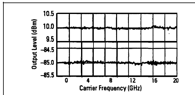
Figure 1-23. Typical Output Level Accuracy and Flatness at + 10 and -85 dBm
