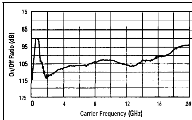
Figure 1-18. Typical Pulse Modulation On/Off Ratio at +8 dBm
