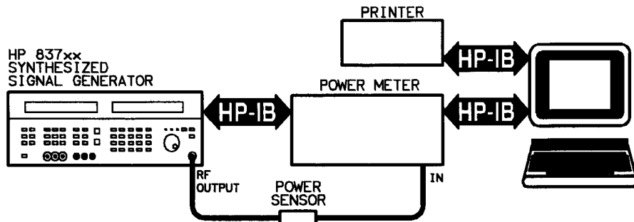
Figure 7-2. 1—20 GHz Vernier Calibration Equipment Setup
