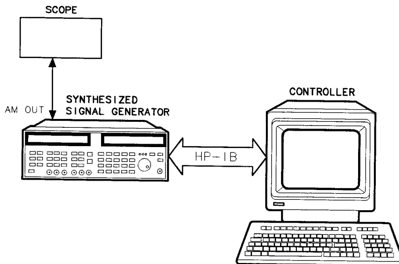
Figure 7-17. Internal Linear AM Source Calibration Equipment Setup
