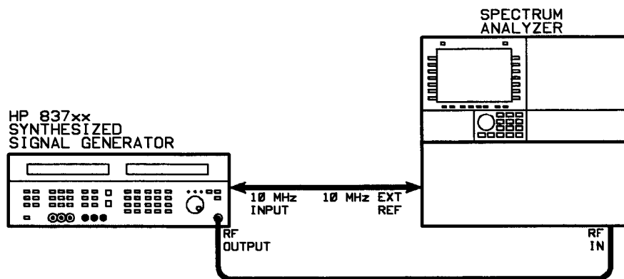
Figure 3-26. Internal AM Rate Test Setup
