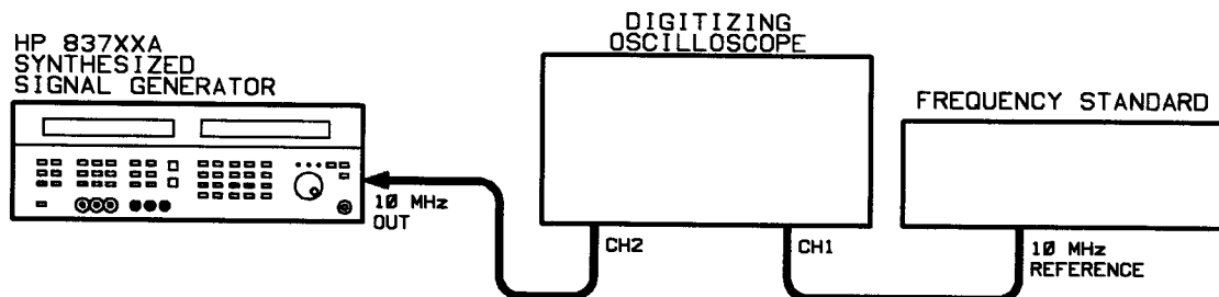
Figure 3-1. Internal Timebase Aging Rate Test Equipment Setup
