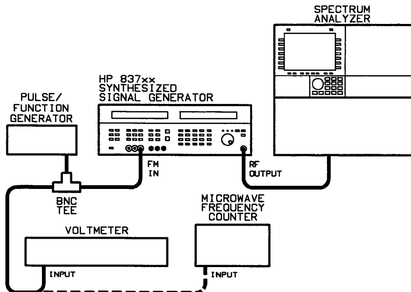
Figure 3-22. FM Rate and Flatness Test Setup
