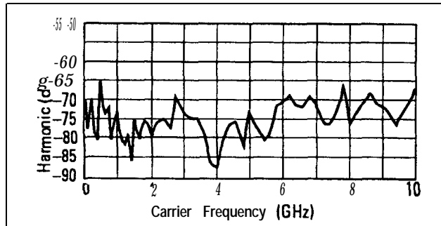
Figure 1-16. Typical 2nd Harmonic Levels Measured at Output Power of +6 dBm
