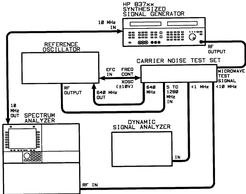
Figure 3-10. Single-Sideband Phase Noise Test Setup
