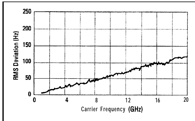
Figure 1-26. Typical Residual FM Measured in 50 Hz – 15 kHz Bandwidth, CW Mode, with High Stability Timebase (Option 1E5)
