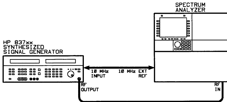
Figure 3-9. Harmonics Test Setup
