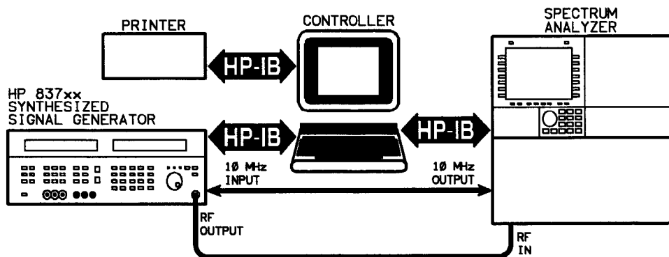
Figure 7-16. Internal AM/FM Source Calibration Equipment Setup
