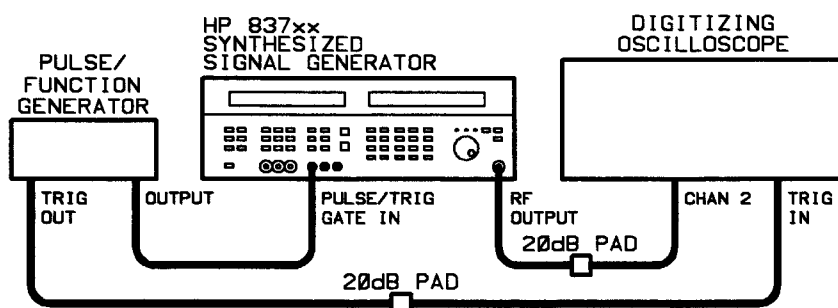
Figure 3-14. Pulse Rise/Fall Time Test Setup
