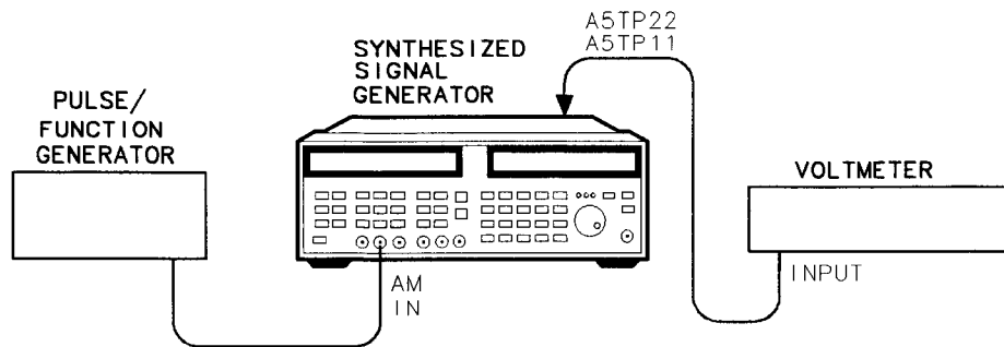
Figure 6-8. Linear AM Offset Equipment Setup
