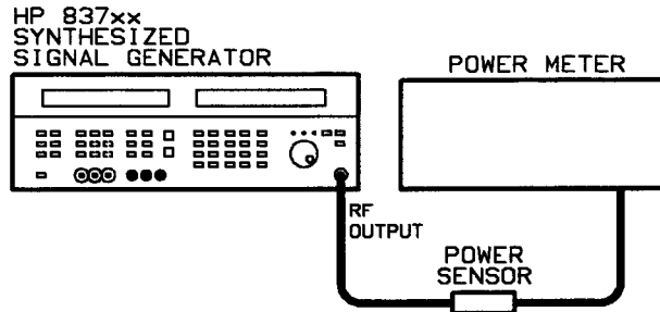
Figure 3-4. Maximum Power Test Setup
