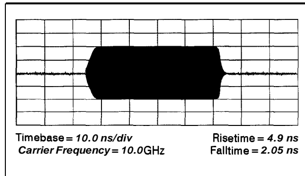
Figure 1-28. Typical Pulse Modulation Envelope Illustrates the Fast Rise and Fall Times, Excellent Flatness and Pulse Fidelity
