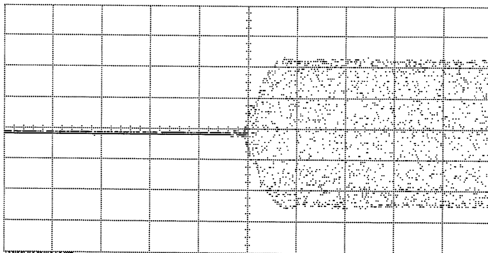
Figure 3-15. Pulse Rise Time Measurement
