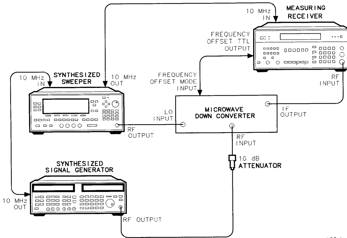
Figure 3-8. 1 GHz to 18 GHz Low Level Accuracy Test Setup using Measuring Receiver
