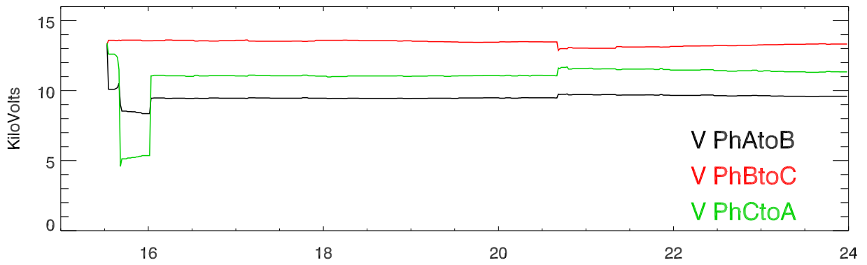
08jun17 AO substation. Phase to Phase voltages vs hour of day
