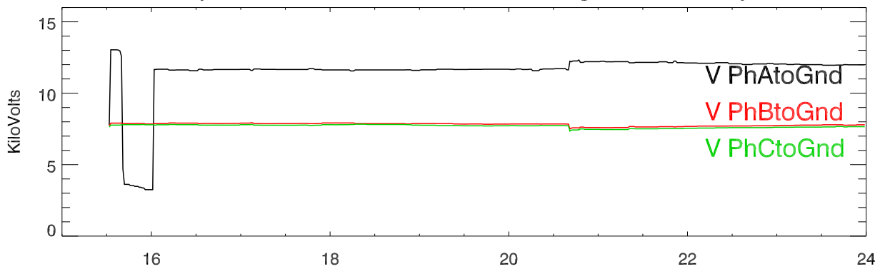
08jun17 AO substation. Phase to Gnd voltages vs hour of day
