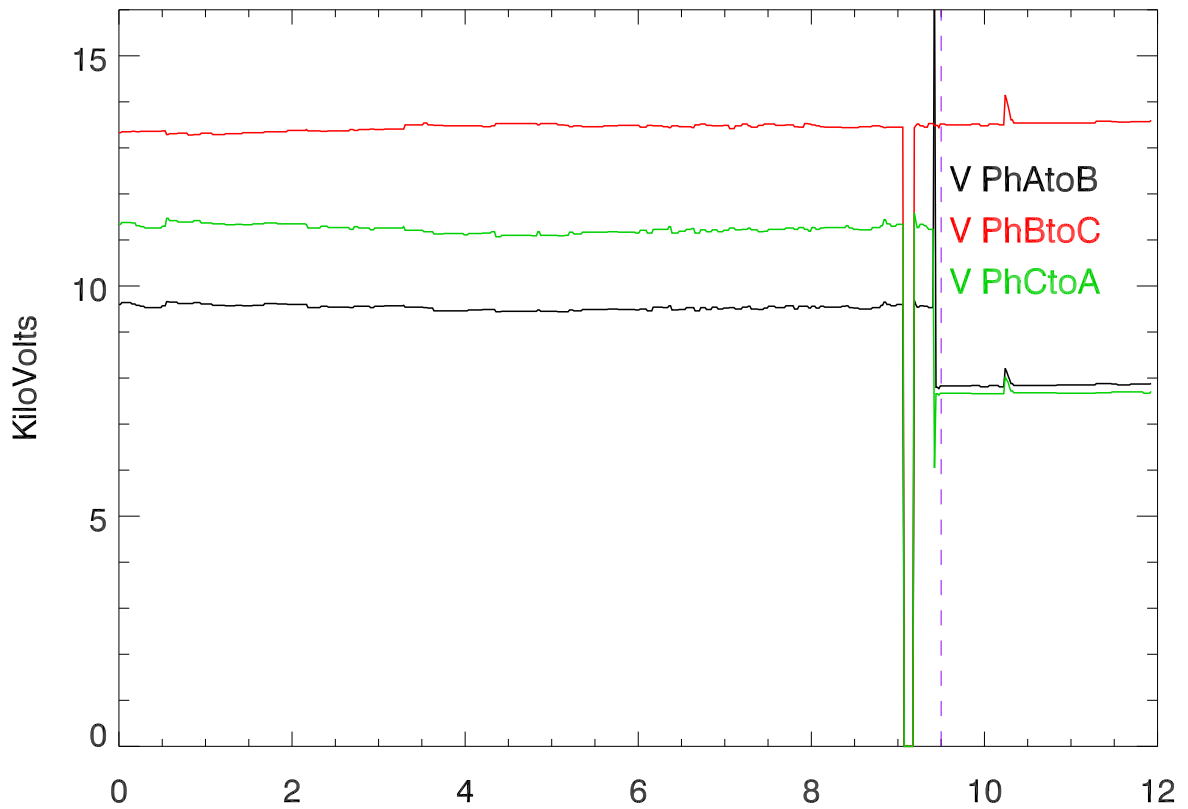
09jun17 AO substation. Phase to Phase voltages vs hour of day
