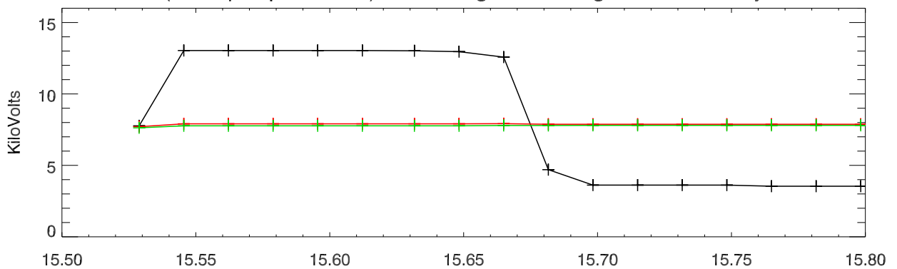
(Blowup at power loss). Phase to ground voltages vs hour of day
