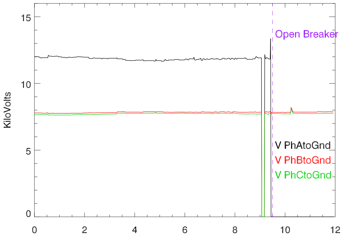
09jun17 AO substation. Phase to Gnd voltages vs hour of day
