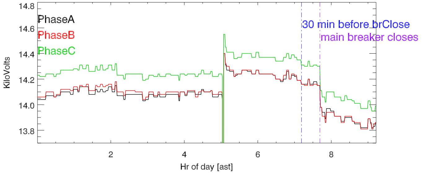
21apr18 site power. PhaseToPhase voltages at breaker input
