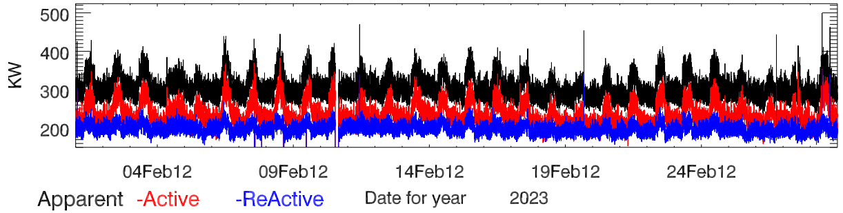
Site power data for feb2023. Power
