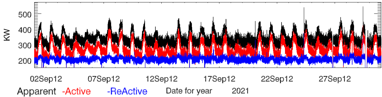
Site power data for sep2021. Power
