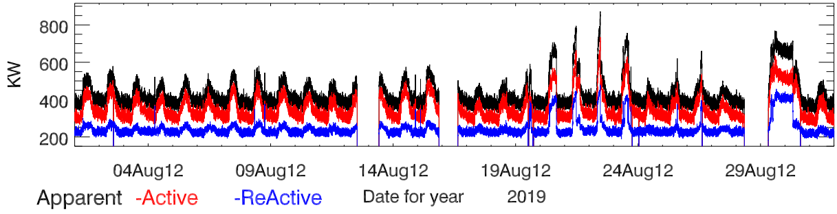
Site power data for aug2019. Power
