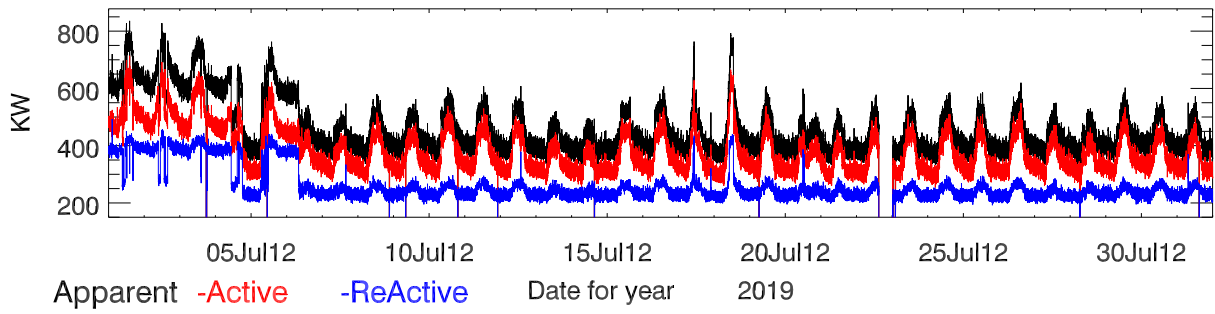
Site power data for jul2019. Power
