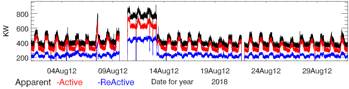
Site power data for aug2018. Power
