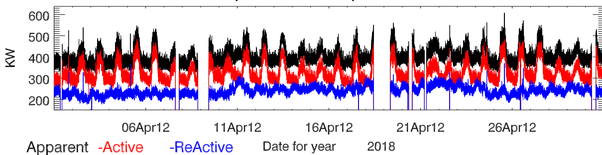
Site power data for apr2018. Power
