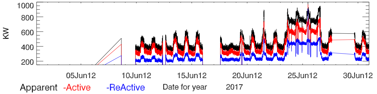
Site power data for jun2017. Power
