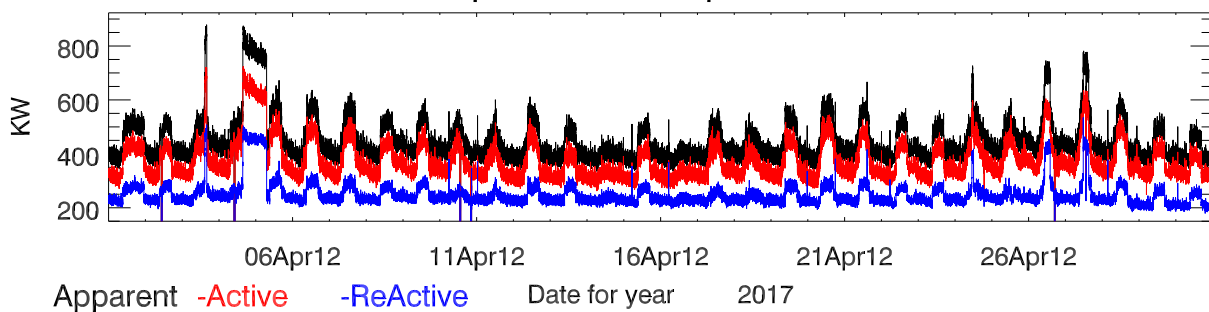
Site power data for apr2017. Power
