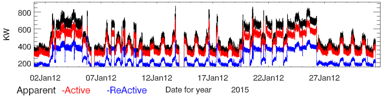
Site power data for jan2015. Power
