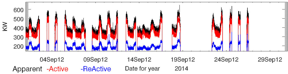
Site power data for sep2014. Power
