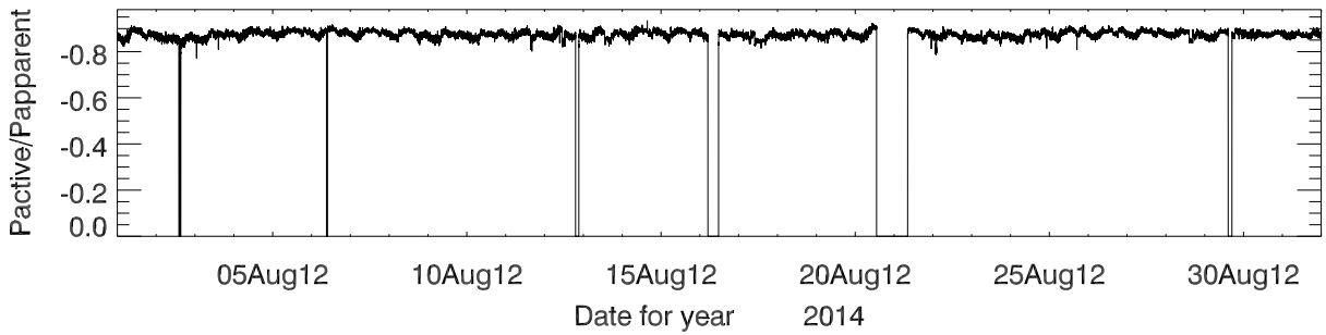
Power factor (computed from Pactive/Papparent)
