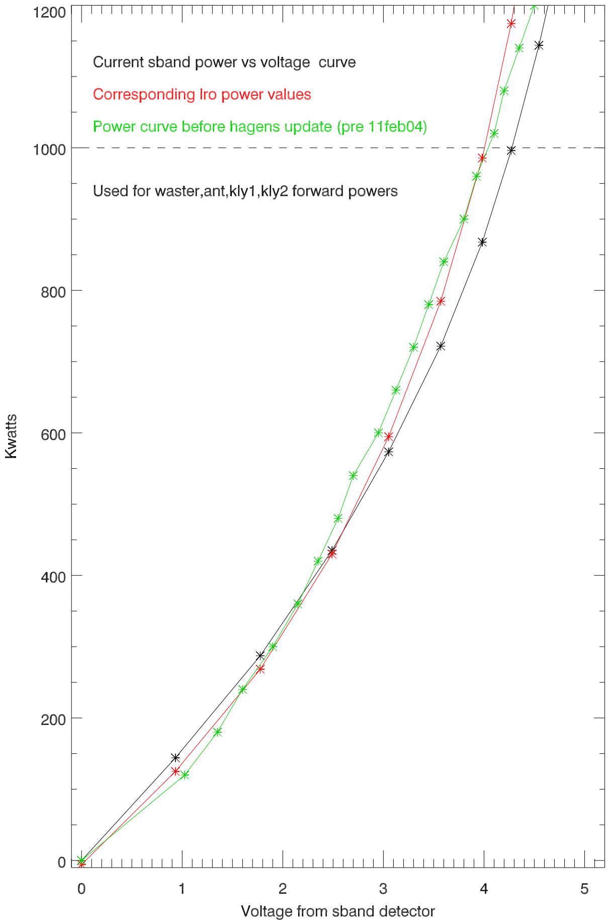
Sband power vs detector voltage (5Volts=fullscale)
