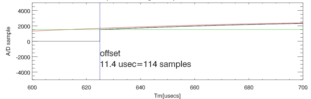
blowup Start of Height samples. data, fit, difference
