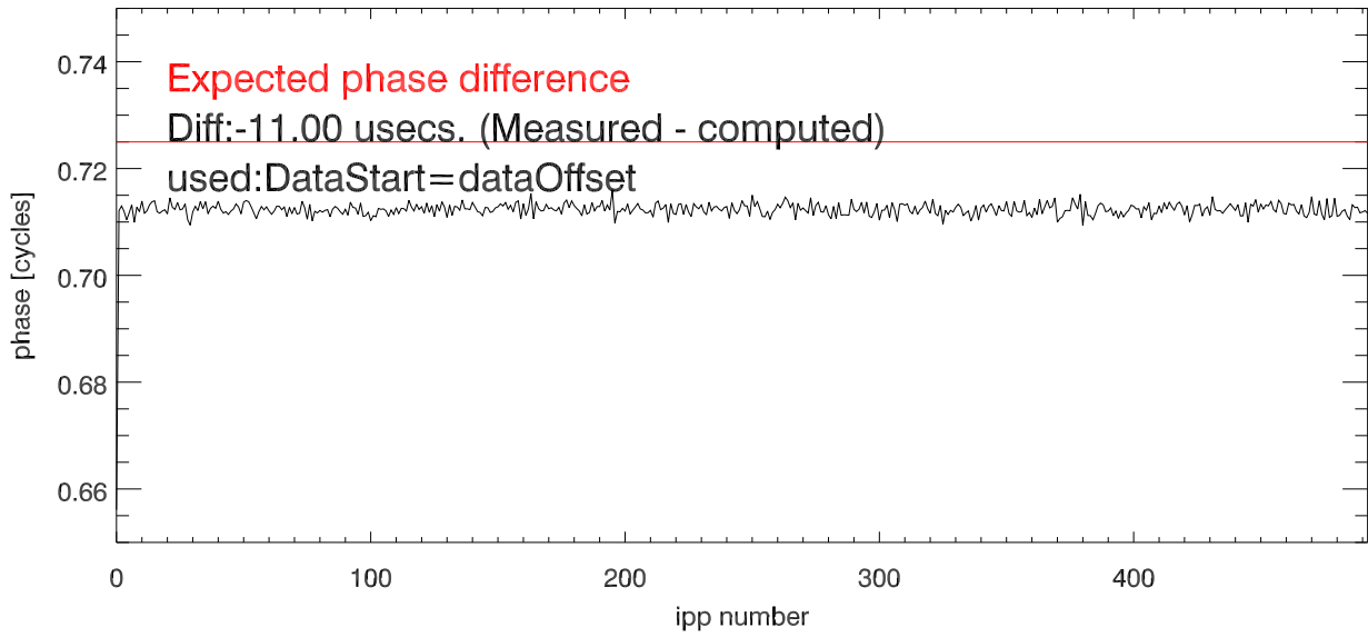
04feb13 phase Data[0,i]-tx[0,i] for each ipp[i]
