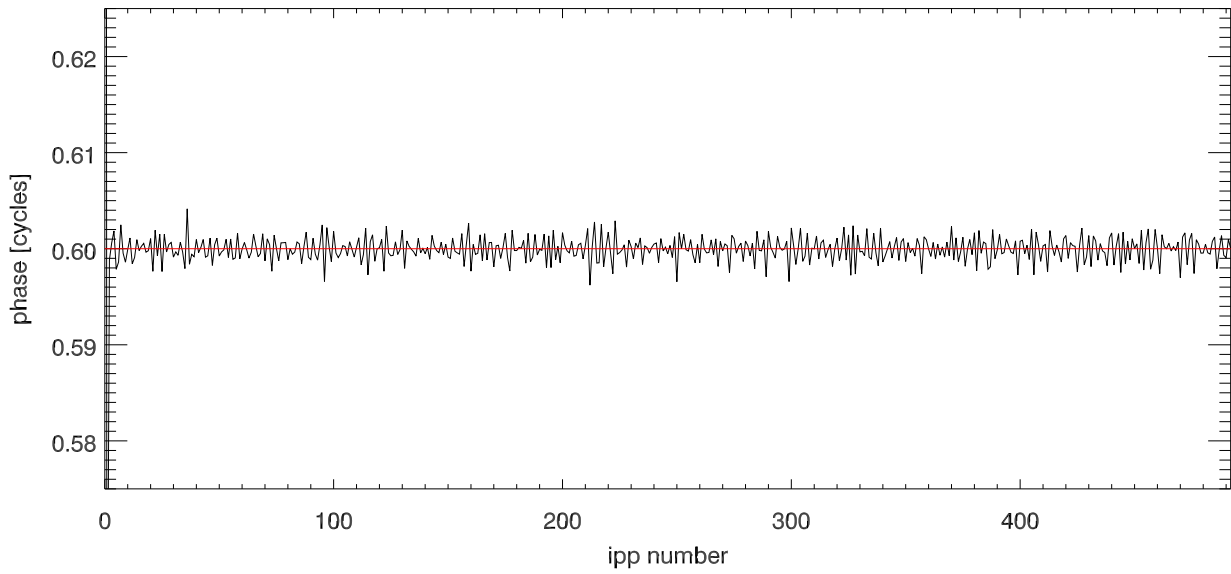
Data Sample[0] phase difference (ipp[n+1]-ipp[n]) vs ipp
