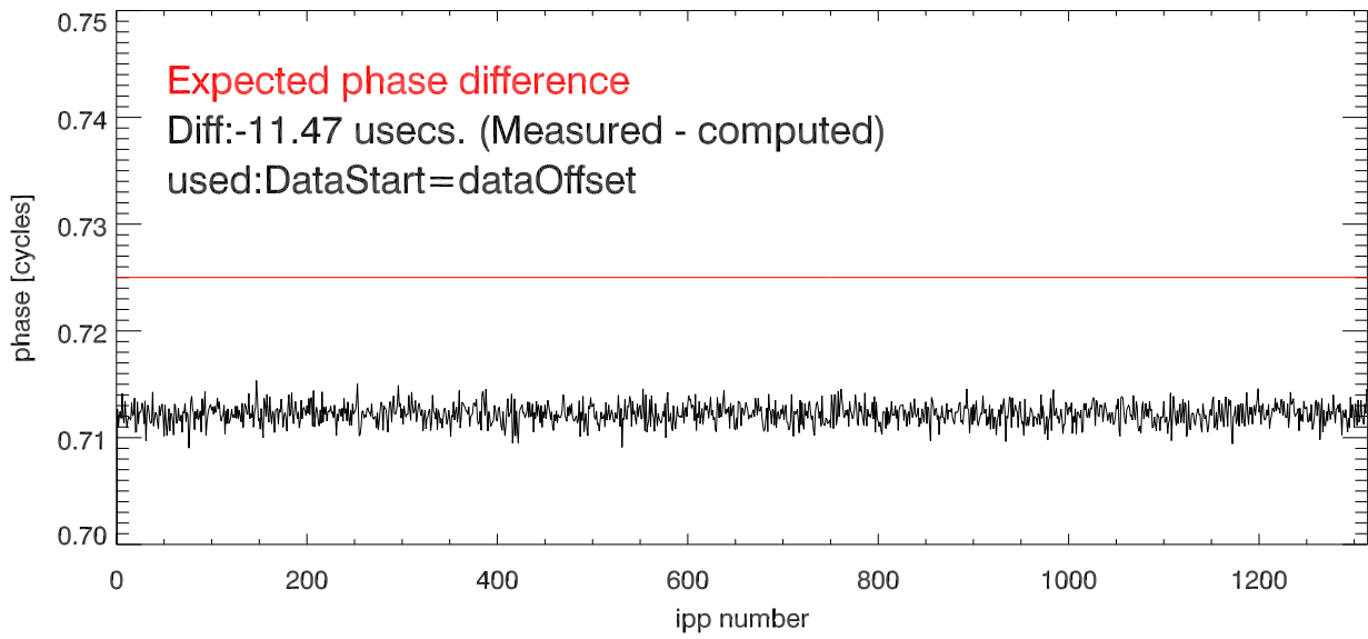
Tx Sample[0] phase difference (ipp[n+1]-ipp[n]) vs ipp
