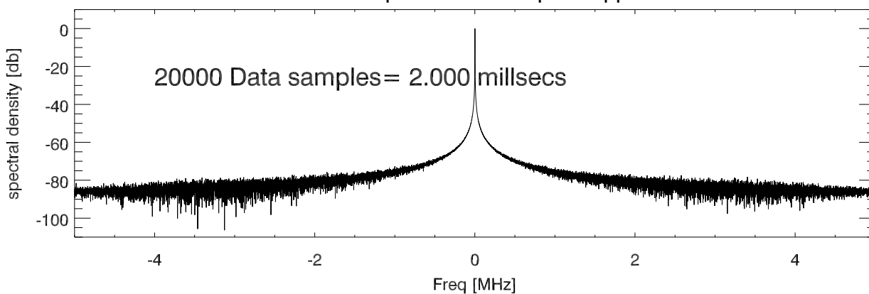
Rdev spectra Data samples 1 ipp
