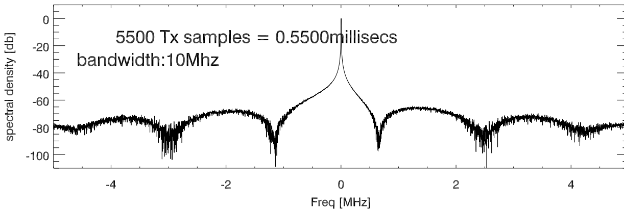
04feb13 Rdev spectra of SineWave frq: 1160:Tx samples 1 ipp.
