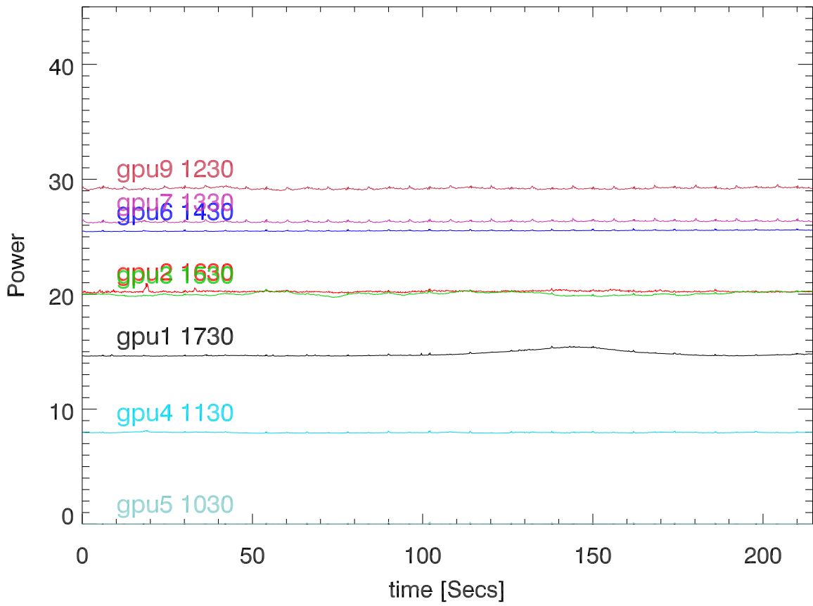
180503 p2789 lbw totalPwr vs Time (by gpu). StokesI
