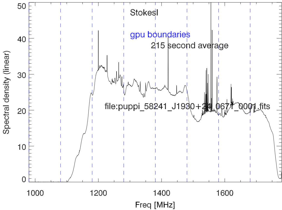
p2789180503 AvgSpectra: puppi_58241_J1930+24_0671_0001.fits
