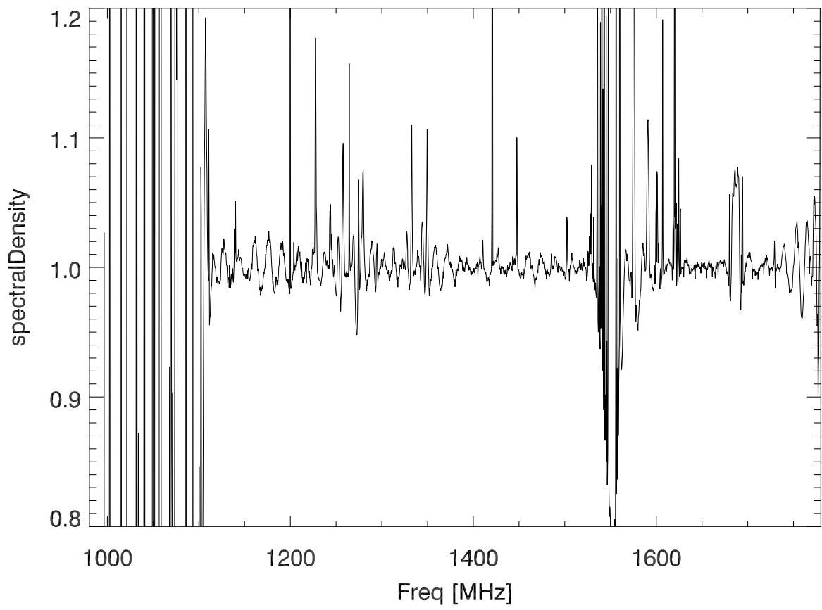
180503p2789 bandPass corrected avgSpc (lbw) StokesI
