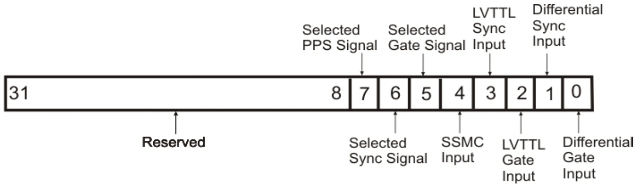
Figure 4-8: Status Register
