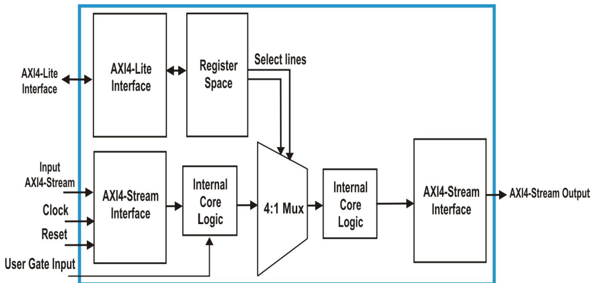
Figure 1-1: AXI4-Stream Gate Substitution Core Block Diagram
