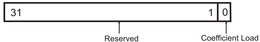
Figure 4-4: Coefficient Load Register
