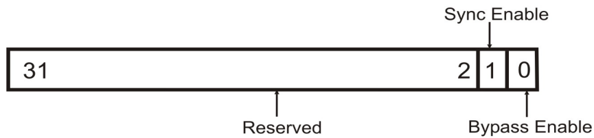
Figure 4-3: Control Register
