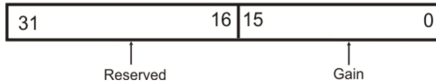
Figure 4-2: Gain Register
