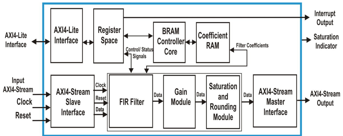
Figure 1-1: AXI4-Stream Folded Symmetrical Decimation FIR Filter Core Block Diagram
