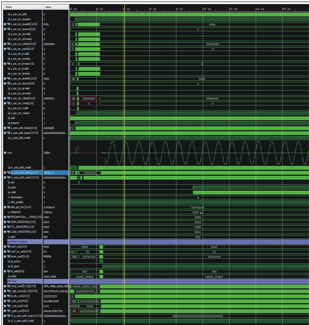
Figure 6-3: AXI4-Stream Folded Symmetrical Decimation FIR Filter Core Test Bench
