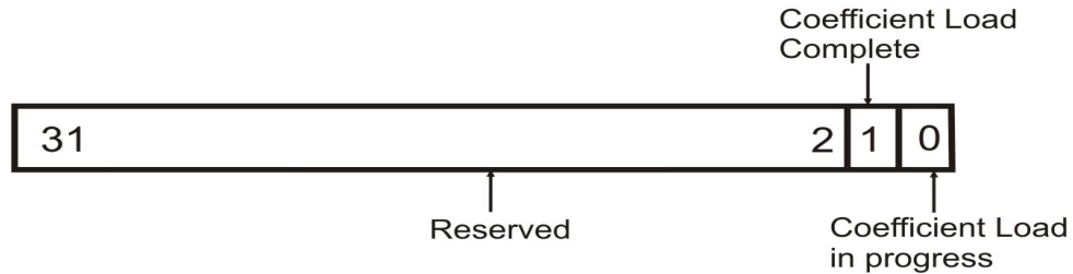
Figure 4-5: Status Register
