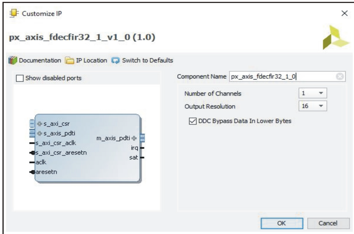
Figure 6-2: AXI4-Stream Folded Symmetrical Decimation FIR Filter Core IP Symbol
