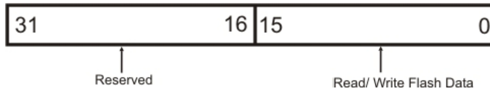
Figure 4-2: Flash Data Register
