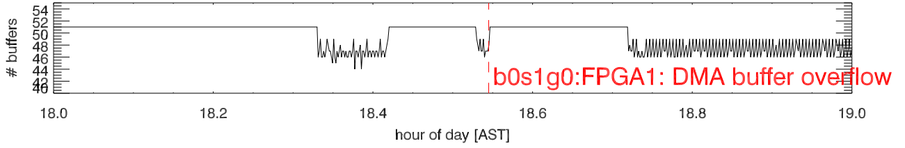
121007 b0g0 Number of free large buffers vs hour
