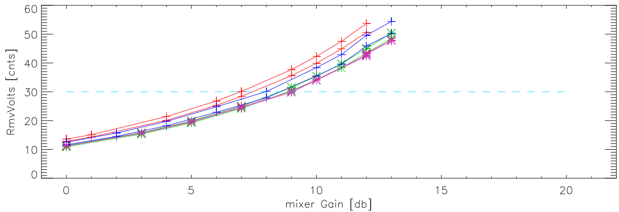
beam2
