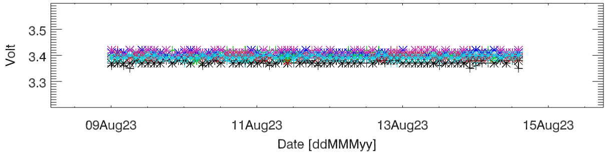
Vdd (3.3V)
