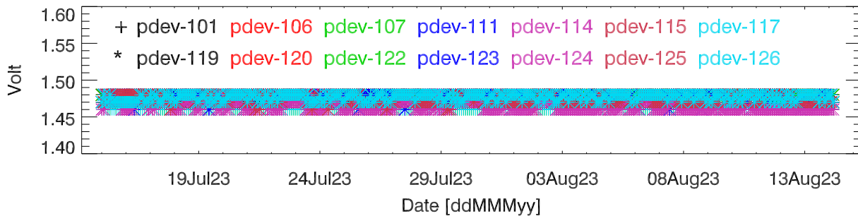
pdev hw last 30 days: Vdd (GxA)
