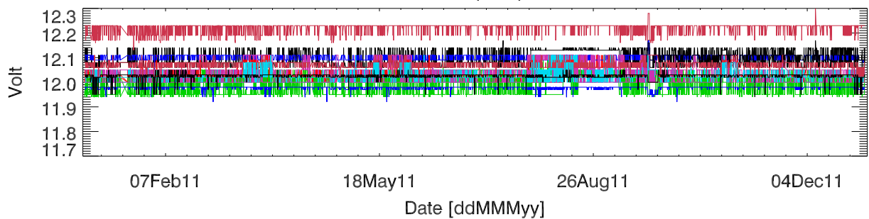
Vdd (12V)
