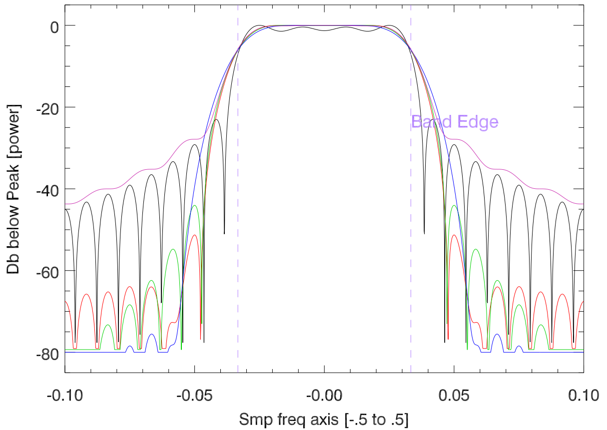
Blowup freq response for mock Digital filters
