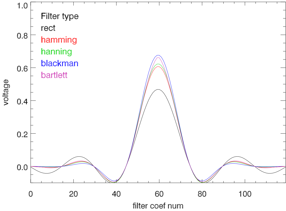
Time domain response Mock digFilt. dec= 15
