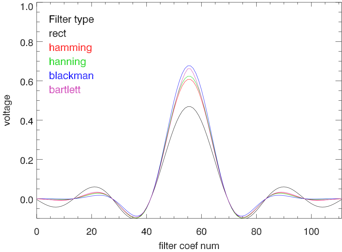
Time domain response Mock digFilt. dec= 14
