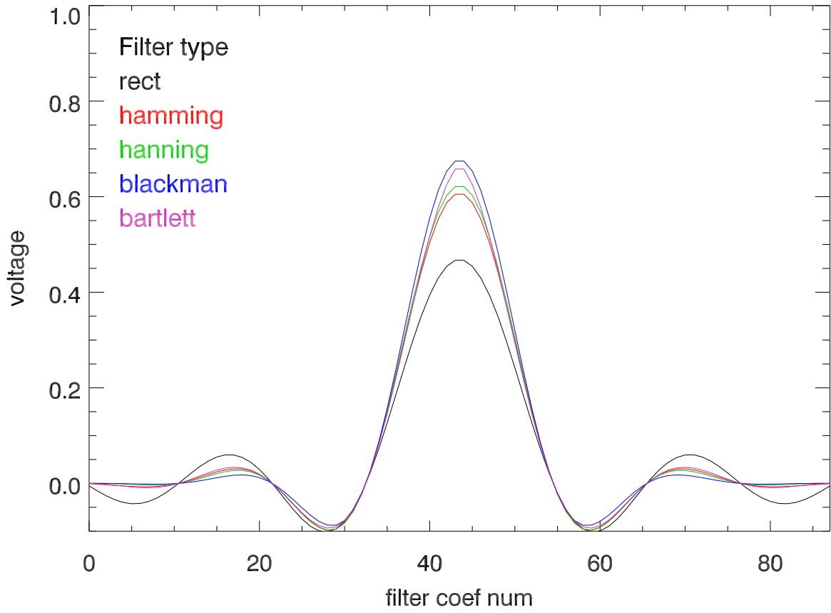
Time domain response Mock digFilt. dec= 11
