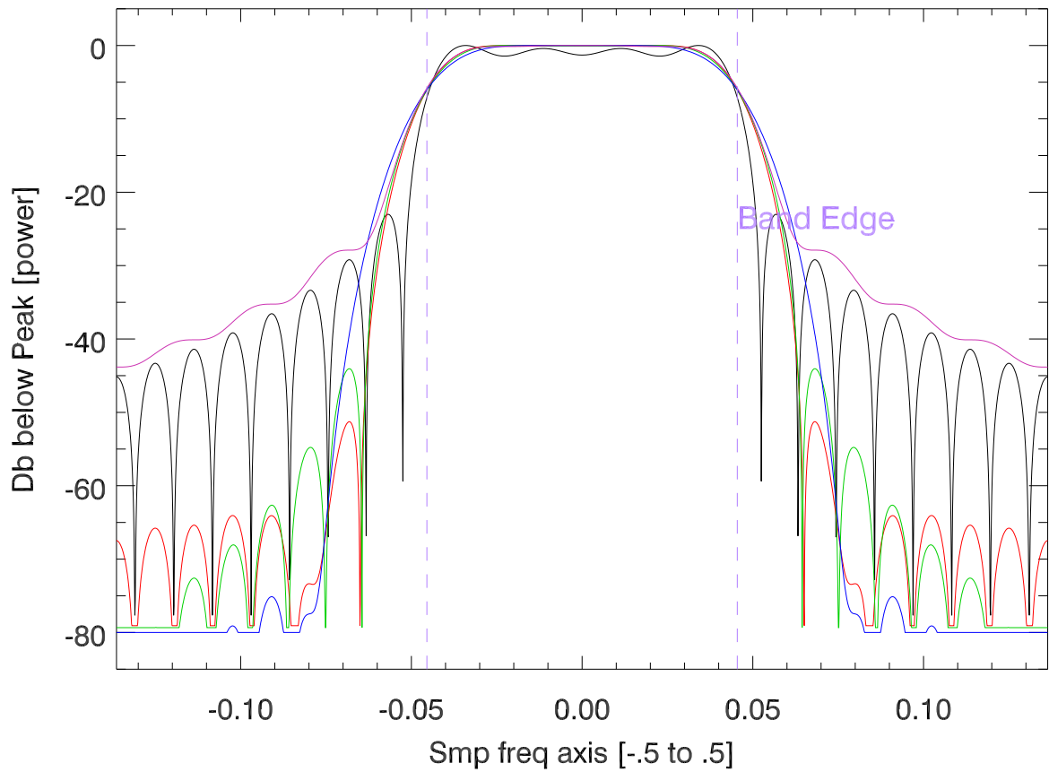
Blowup freq response for mock Digital filters
