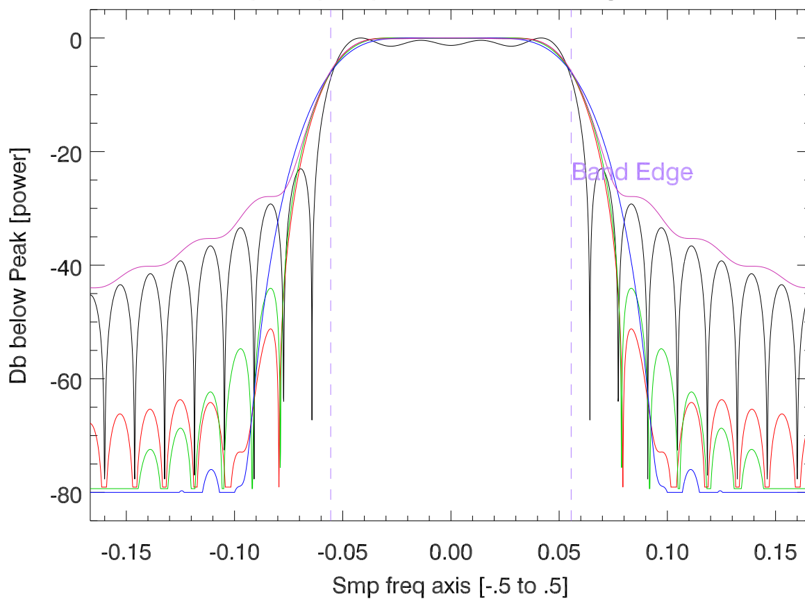
Blowup freq response for mock Digital filters
