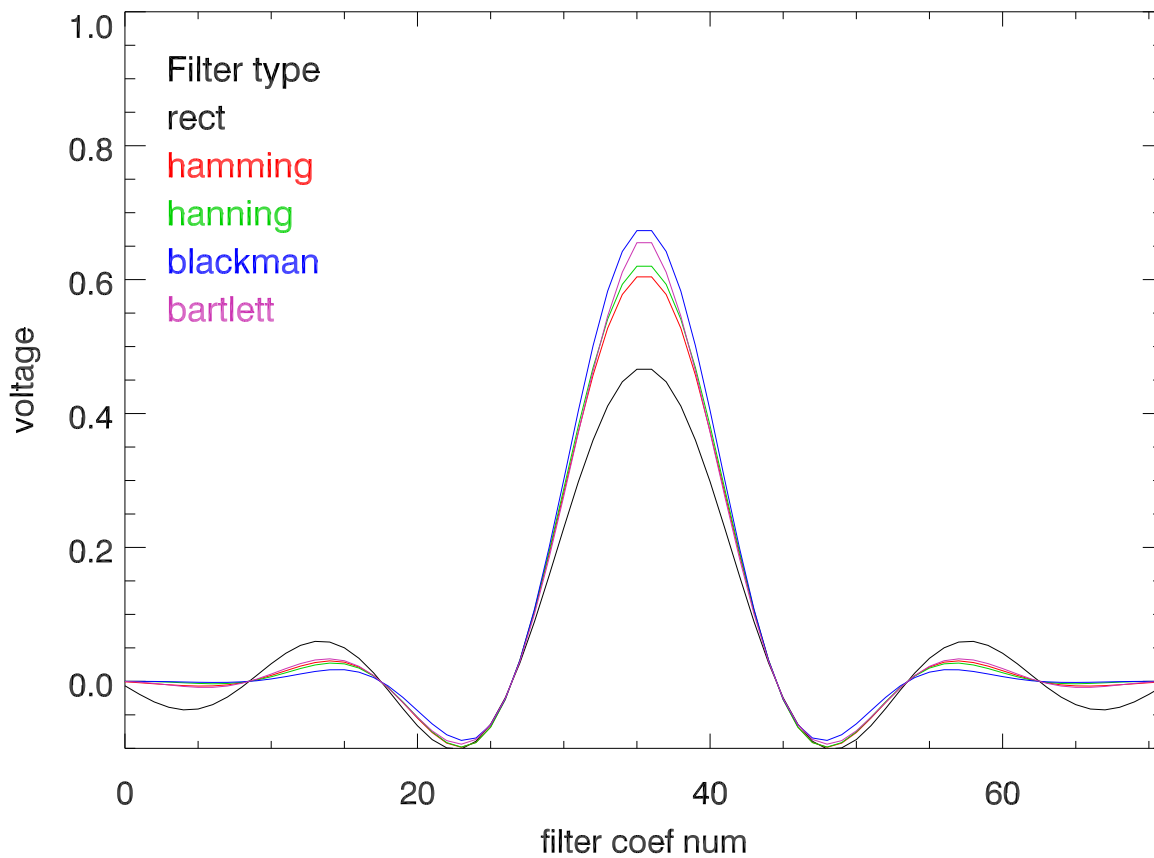
Time domain response Mock digFilt. dec= 9
