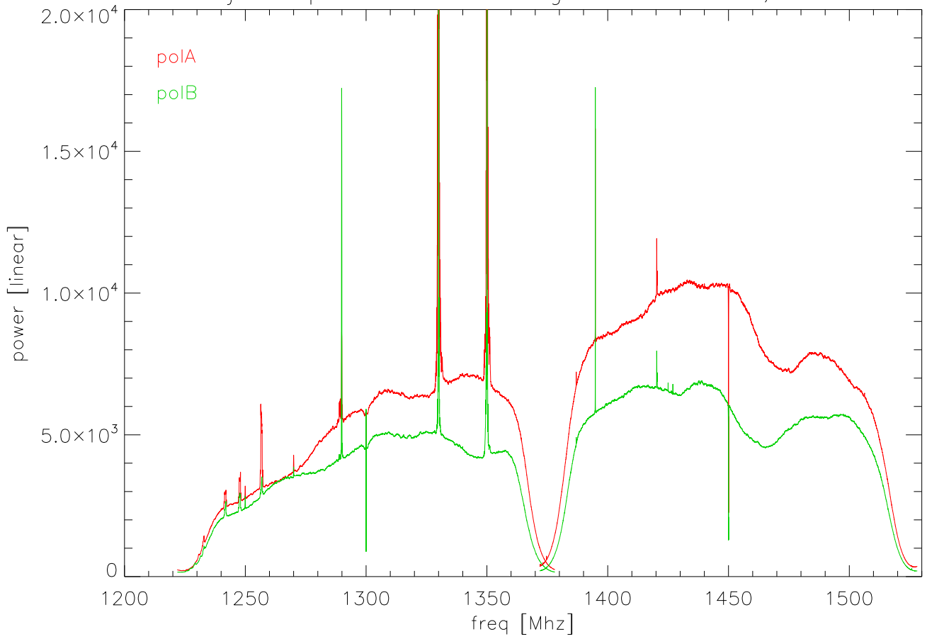
22jan07 pdevs0 20 sec integration at az=10,za=18
