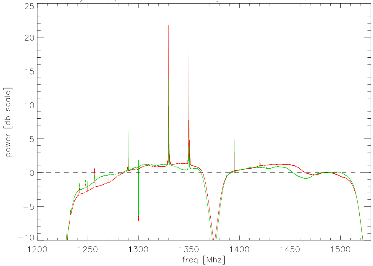
22jan07 pdevs0 20 sec integration at az=10,za=18
