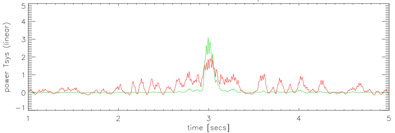
1300 Mhz band blowup
