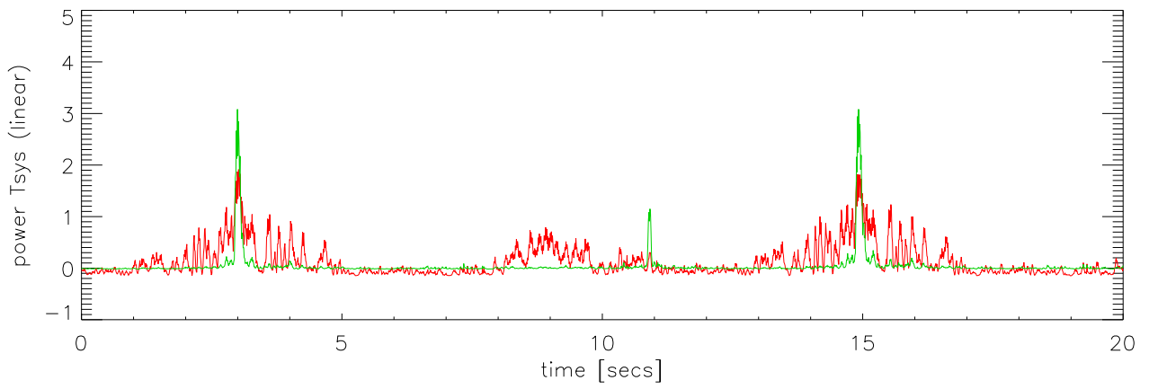
1450 Mhz band blowup
