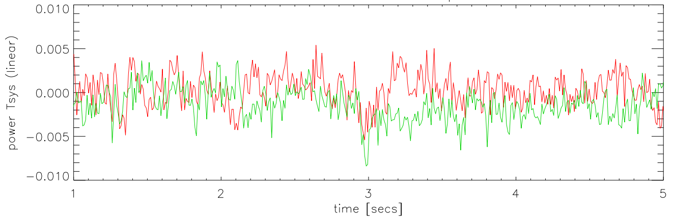
1300 Mhz band blowup
