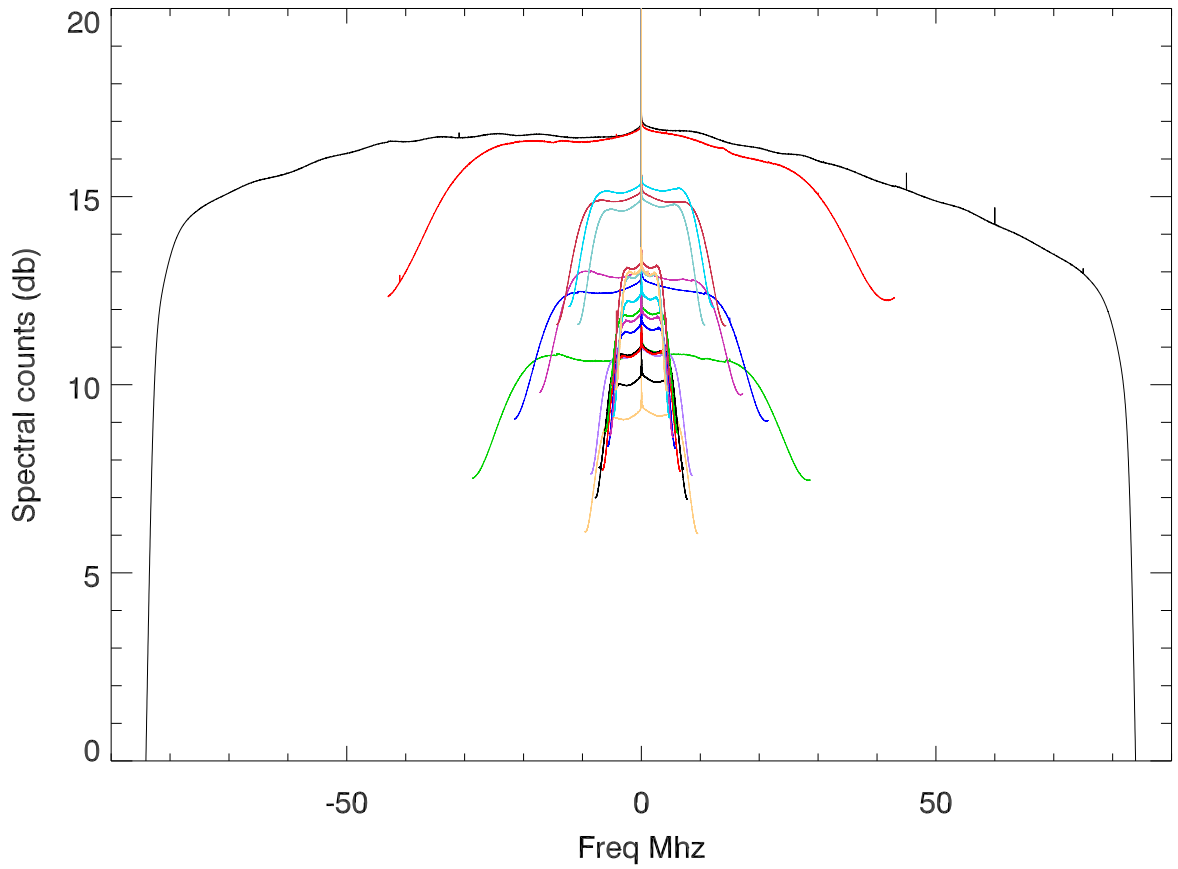
Spectral density for Single accumulation (1fft). dec 1..20
