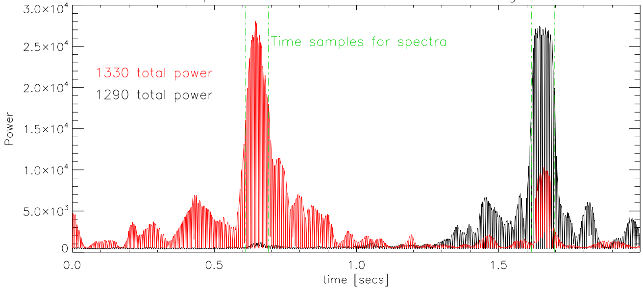
Spectral density for 1330 MhzPk
