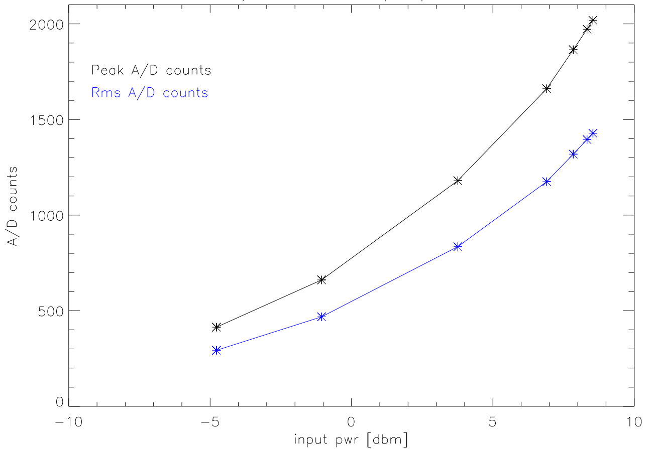
A/D counts vs input power
