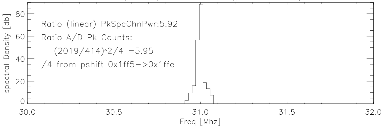
Blowup Pk A/D=414 cnts (pshift=0x1ff5)
