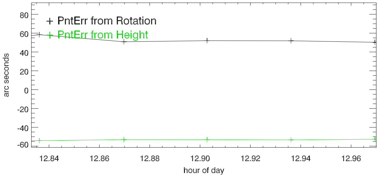
190919 point error from platform rotation and vertical motion
