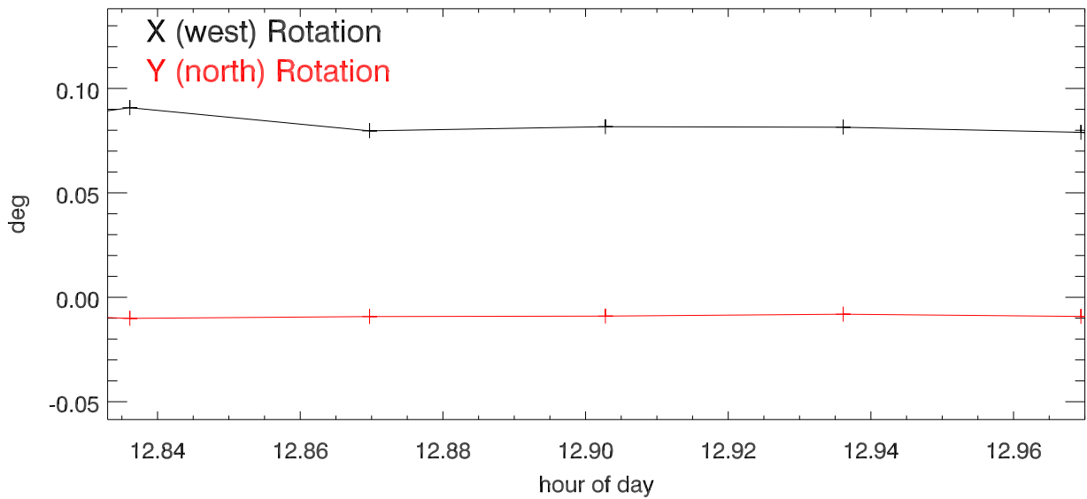
190919 Extra platform rotations (current - model)
