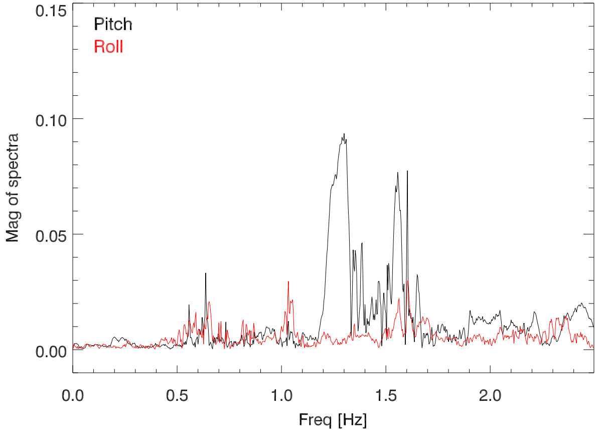
Magnitude of tilt sensor spectra around earthquake
