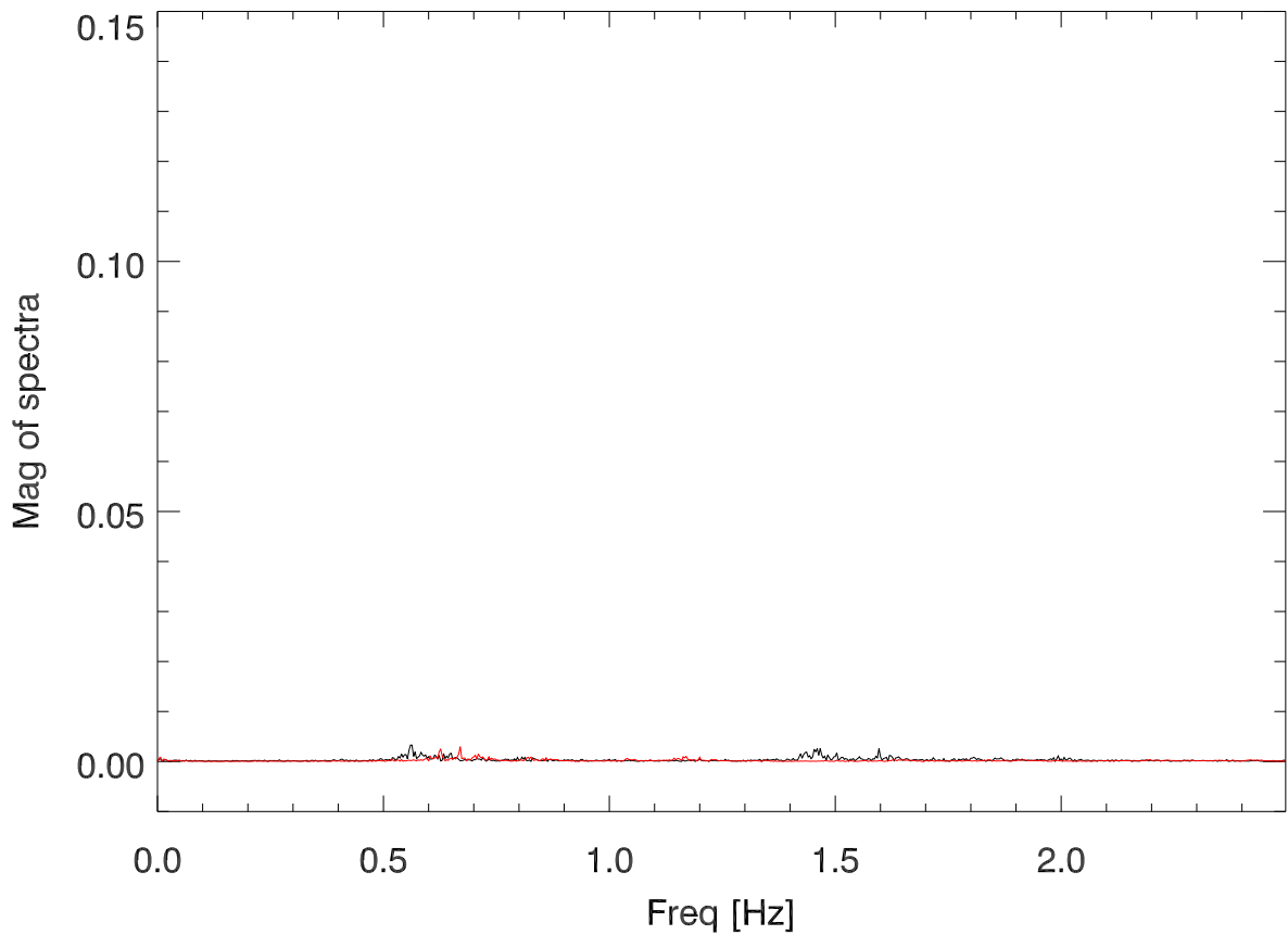
Magnitude of tilt sensor spectra before earthquake
