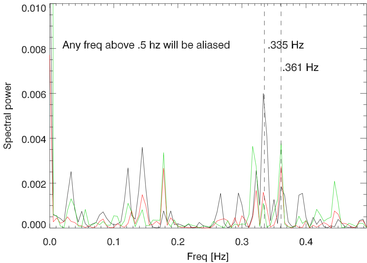
Spectrum of tdTension oscillations
