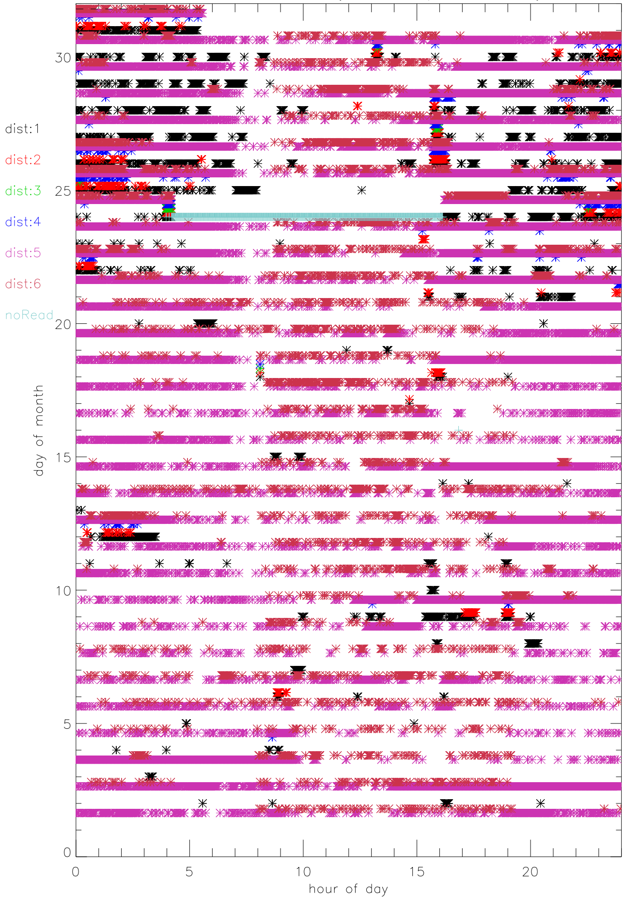
distomat failures for may18 last updated:31may18
