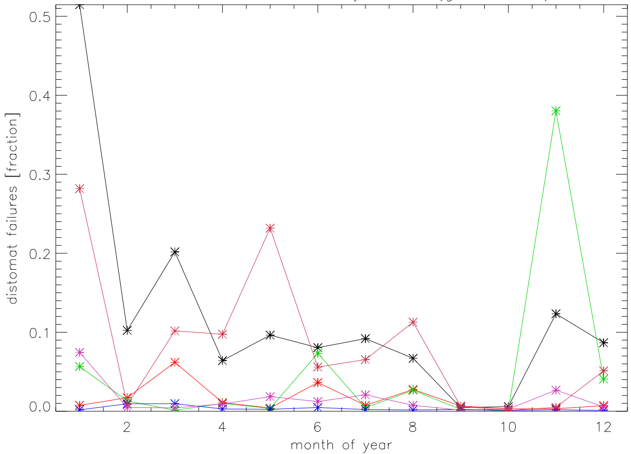
2020 distomat failures by month (gooddist=3)
