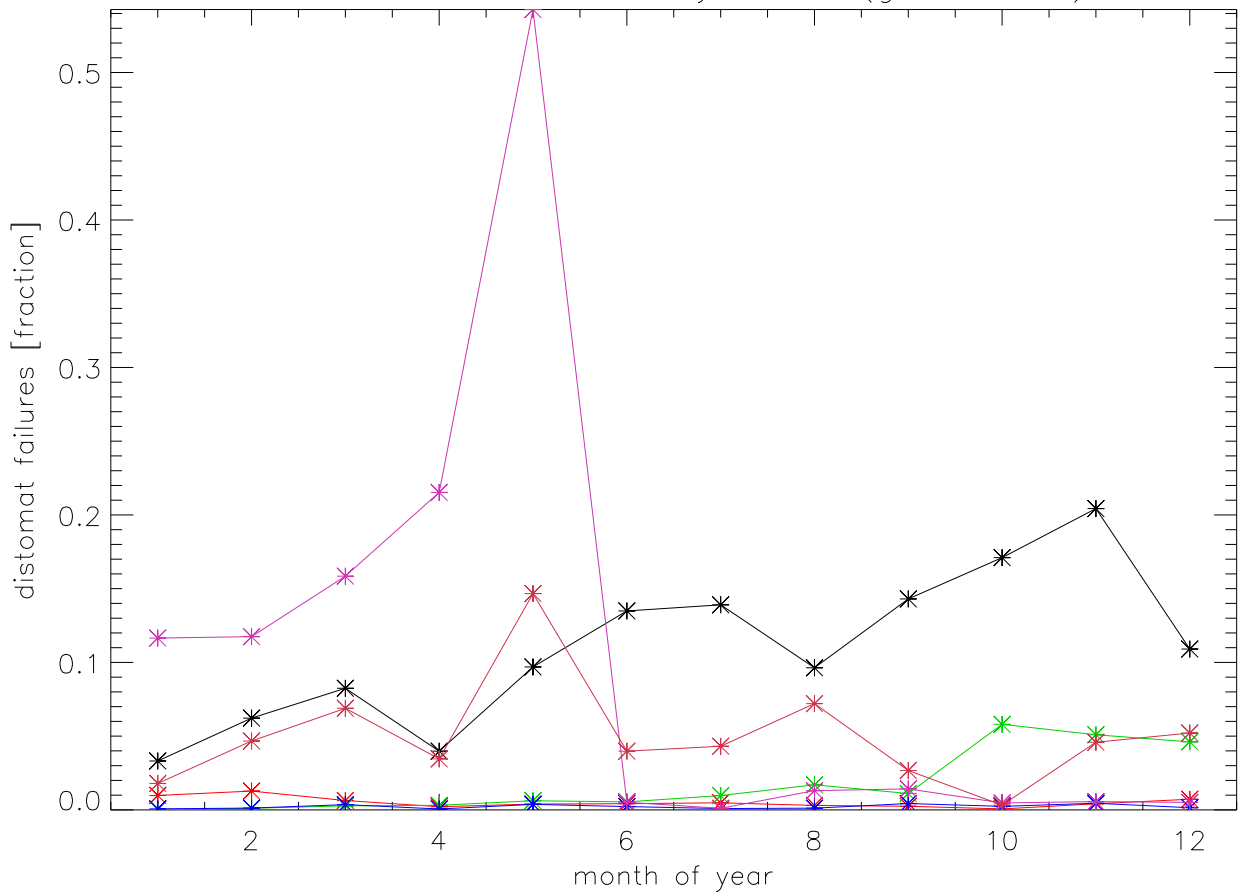
2019 distomat failures by month (gooddist=3)
