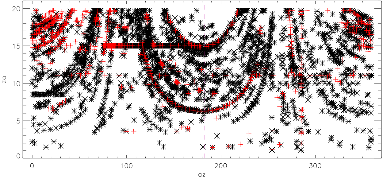
feb 2017 distomats 2,3 failures (T4) * DIST2 + DIST3
