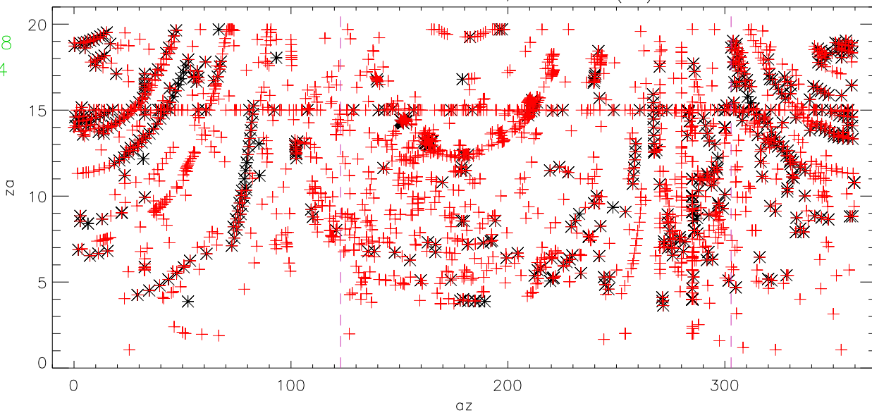
nov 2013 distomats 4,5 failures (T8) * DIST4 + DIST5
